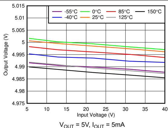
5-6. Line Regulation vs V_{IN} (New Chip)
