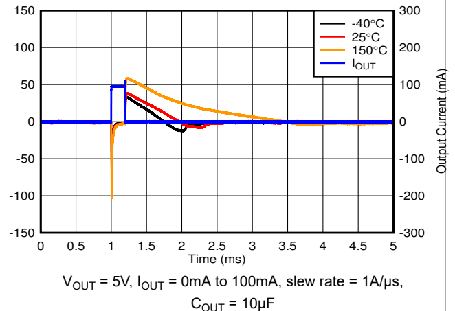
FIG 5-30. Load Transient, No Load to 100mA (New Chip)
