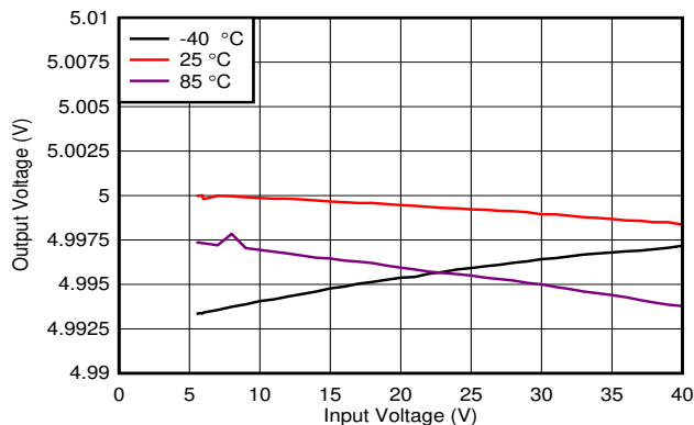
Figure 5-7. Line Regulation vs V_{IN} (New Chip)
