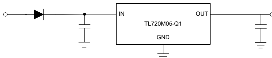
図 8-5. Typical Application Diagram (New Chip)
