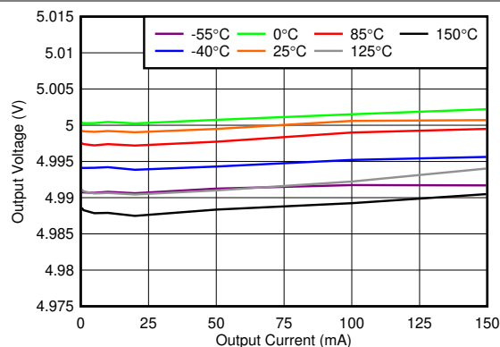
Figure 5-8. Load Regulation vs I_{OUT} (New Chip)
