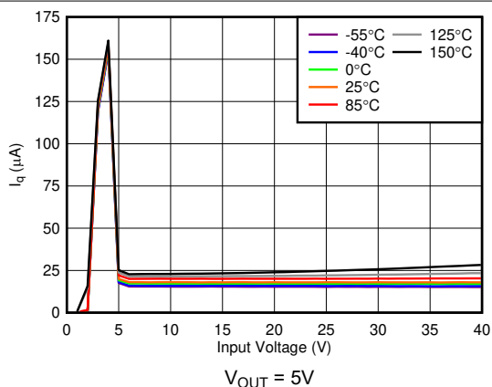
FIG 5-15. Quiescent Current ( I_Q ) vs V_{IN} (New Chip)
