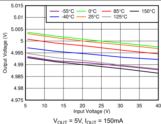
5-5. Line Regulation vs V_{IN} (New Chip)
