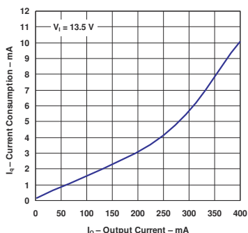
FIG 5-13. Current Consumption vs Output Current (Legacy Chip)
