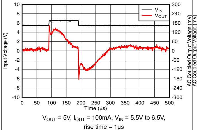
FIG 5-29. Line Transients (New Chip)
