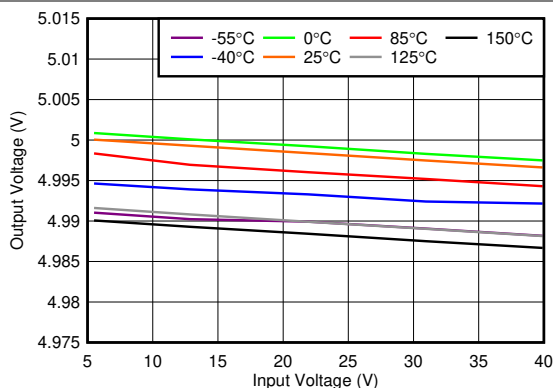
Figure 5-7. Line Regulation vs V_{IN} (New Chip)
