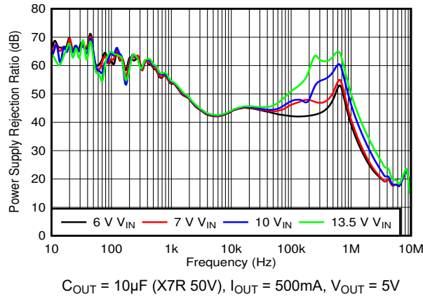
FIG 5-25. Power-Supply Ripple Rejection vs Frequency and V_{IN} (New Chip)
