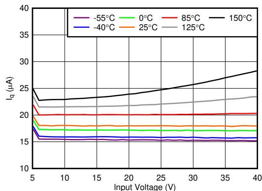
FIG 5-14. Quiescent Current ( I_Q ) vs V_{IN} (New Chip)
