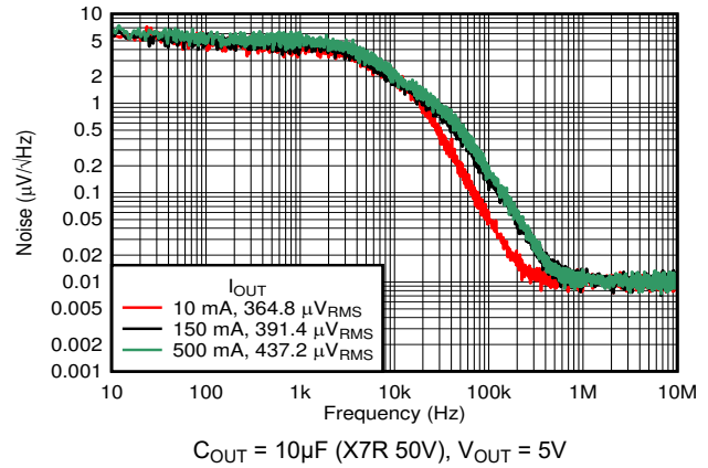
FIG 5-26. Noise vs Frequency (Legacy Chip)
