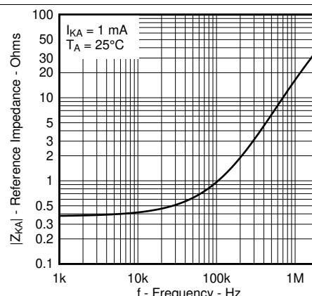
FIG 8. Reference Impedance versus Frequency
