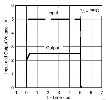
FIG 10. Pulse Response
