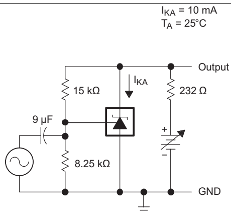
FIG 7. Test Circuit for Voltage Amplification
