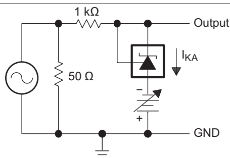
FIG 7. Test Circuit for Voltage Amplification
