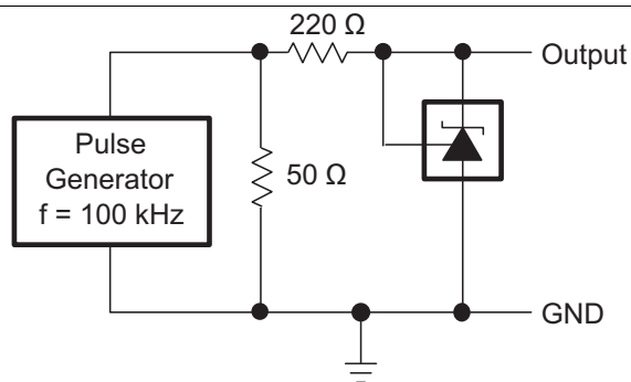
FIG 9. Test Circuit for Reference Impedance
