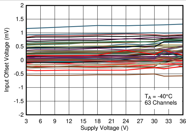
FIG 5-11. Input Offset Voltage vs. Supply Voltage at -40^\circ\text{C}
