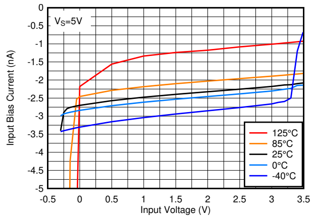
FIG 5-8. Input Bias Current vs. Input Voltage at 5V
