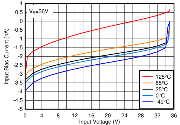
FIG 5-10. Input Bias Current vs. Input Voltage at 36V
