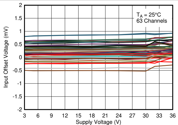
FIG 5-12. Input Offset Voltage vs. Supply Voltage at 25^\circ\text{C}
