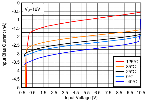
FIG 5-9. Input Bias Current vs. Input Voltage at 12V
