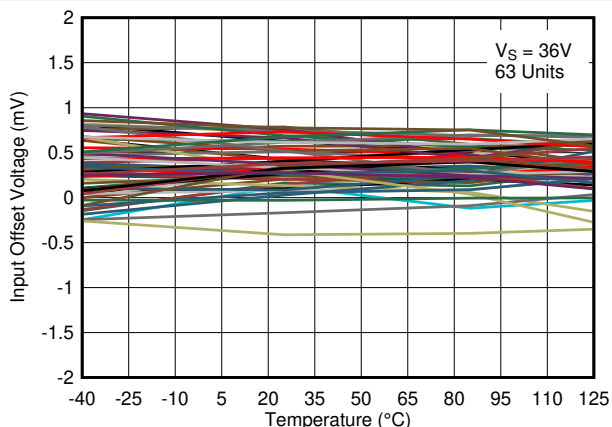
5-18. Input Offset Voltage vs. Temperature at 36V
