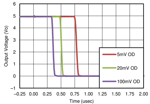
7-3. Response Time for Various Overdrives (Negative Transition)
