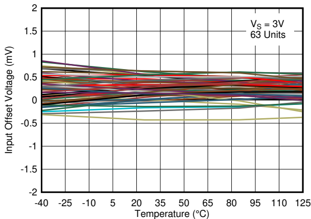
5-15. Input Offset Voltage vs. Temperature at 3V
