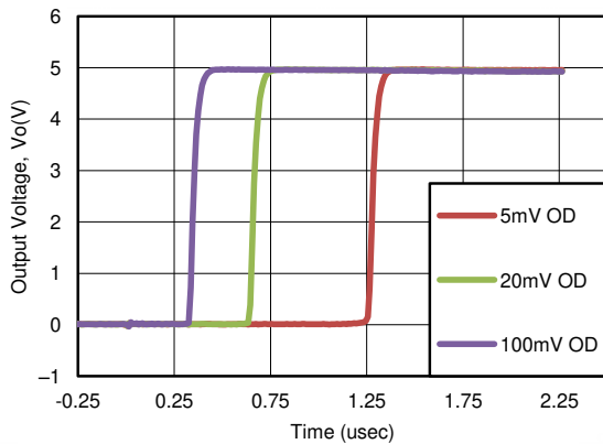
7-2. Response Time for Various Overdrives (Positive Transition)
