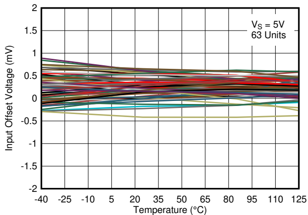
5-16. Input Offset Voltage vs. Temperature at 5V
