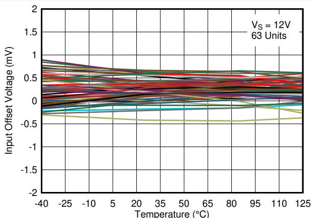
5-17. Input Offset Voltage vs. Temperature at 12V
