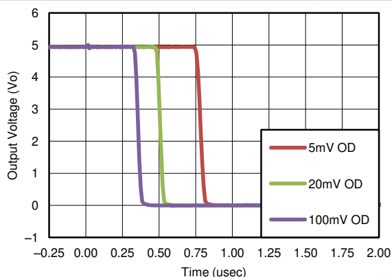
7-3. Response Time for Various Overdrives (Negative Transition)
