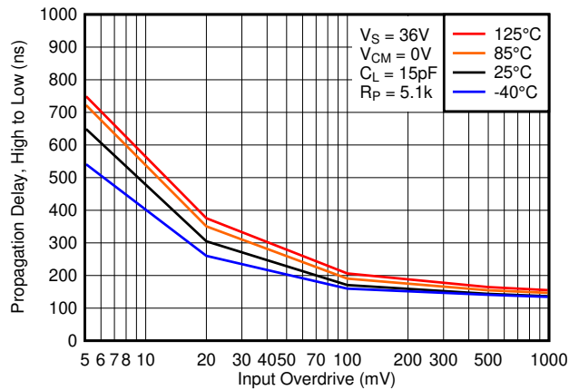
FIG 5-29. High to Low Propagation Delay vs. Input Overdrive Voltage, 36V
