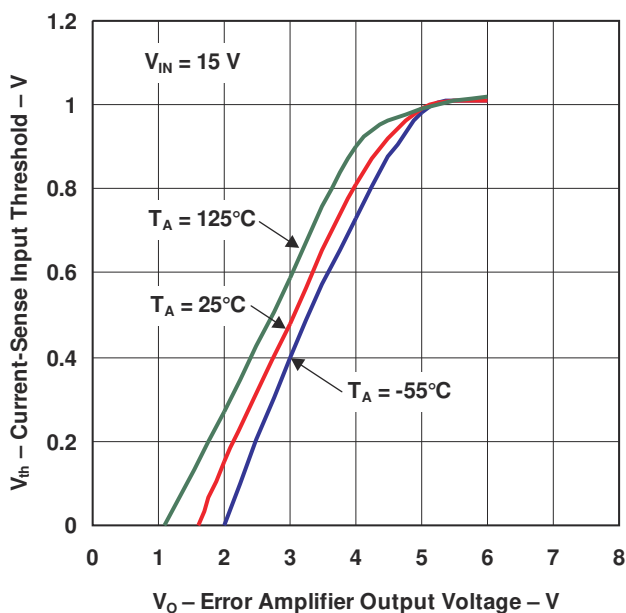
図 5-3. Current-Sense Input Threshold vs Error Amplifier Output Voltage
