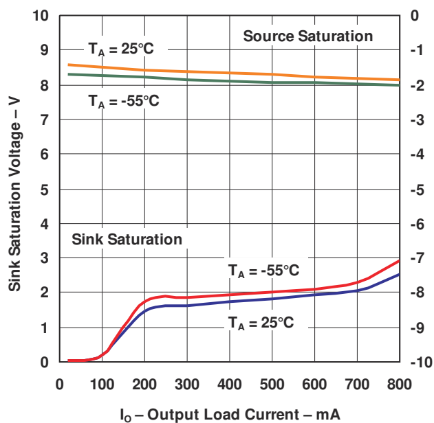
図 5-8. Output Saturation Voltage vs Load Current
