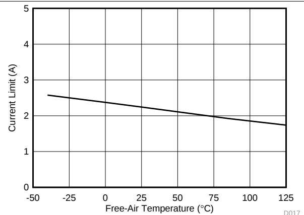
Figure 20. Current Limit vs Temperature
