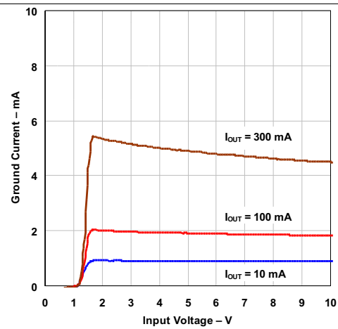
Figure 10. Ground Current vs Input Voltage
