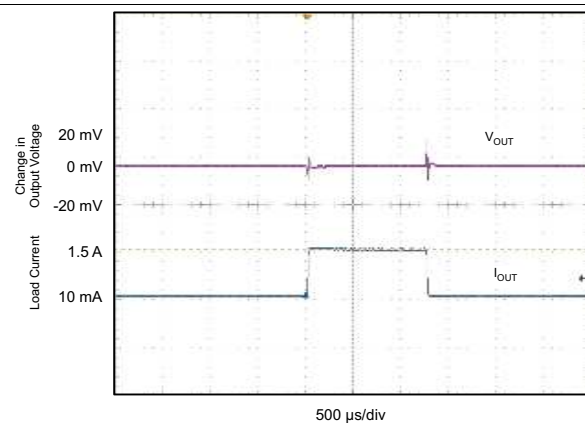
Figure 26. Load Transient Response
