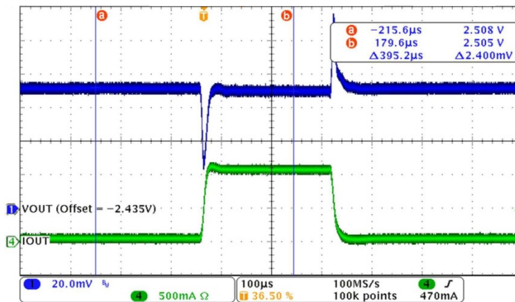
Figure 33. 1-A Load Transient Response ( C_{OUT} = 10 \mu F )
