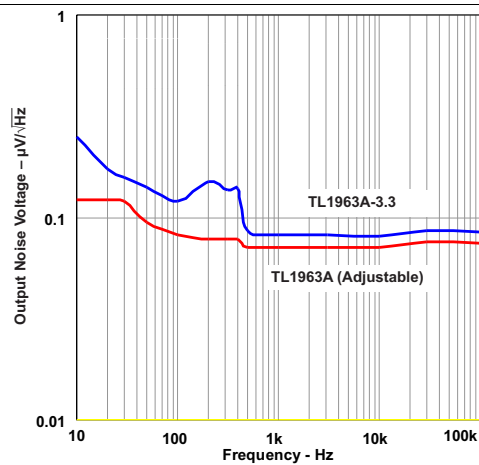
Figure 25. Output Noise Voltage vs Frequency
