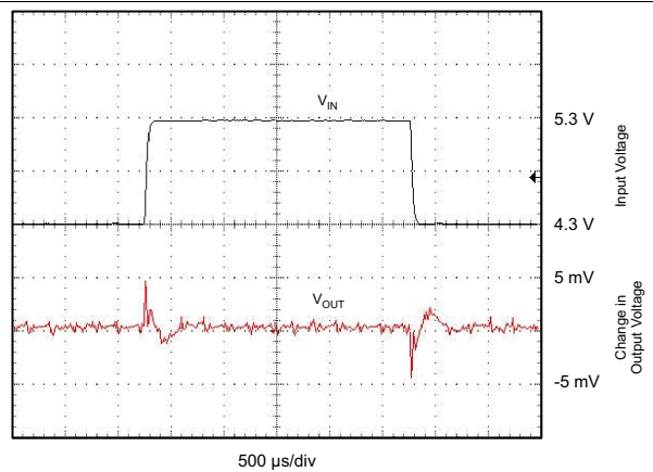
Figure 28. Line Transient Response
