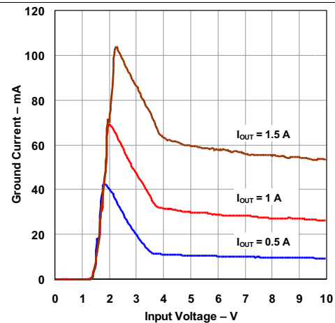
Figure 12. Ground Current vs Input Voltage
