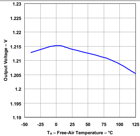
Figure 7. Output Voltage vs Temperature
