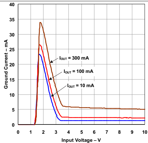
Figure 11. Ground Current vs Input Voltage
