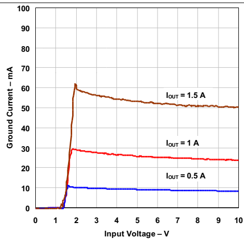
Figure 9. Ground Current vs Input Voltage
