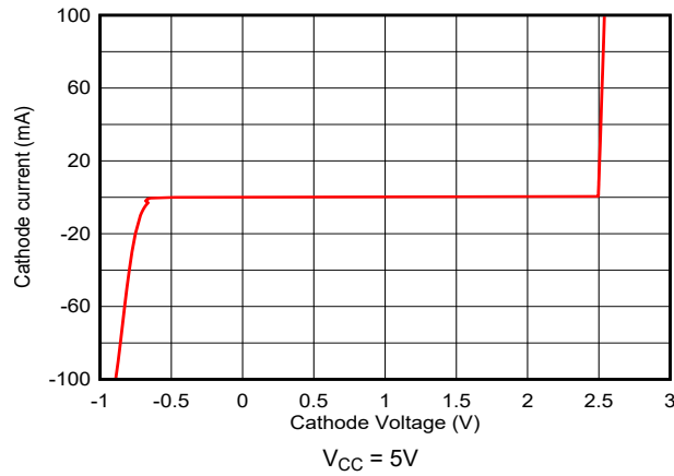
図 5-19. Cathode Current vs Cathode Voltage
