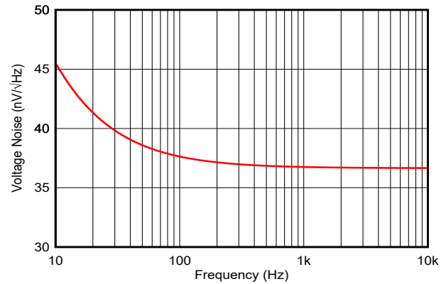
FIG 5-14. Input Voltage Noise Spectral Density vs Frequency
