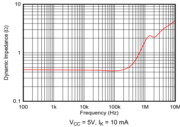
図 5-21. Reference Dynamic Impedance vs Frequency
