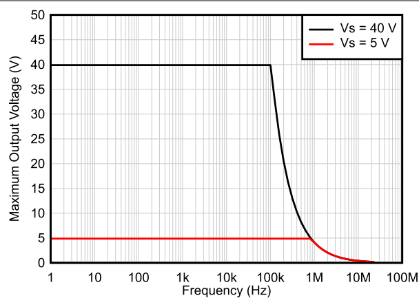
Figure 5-37. Maximum Output Voltage vs Frequency
