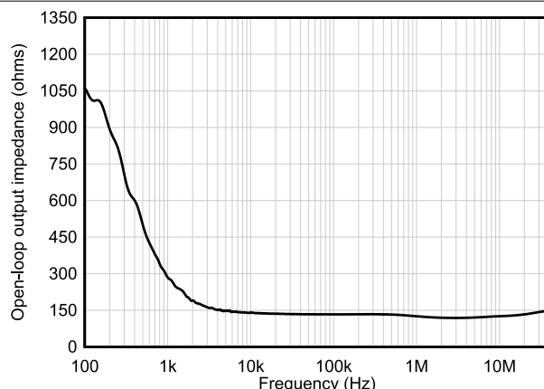
FIG 5-24. Open-Loop Output Impedance vs Frequency
