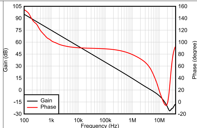
図 5-8. Open-Loop Gain and Phase vs Frequency
