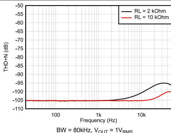
FIG 5-19. THD+N Ratio vs Frequency
