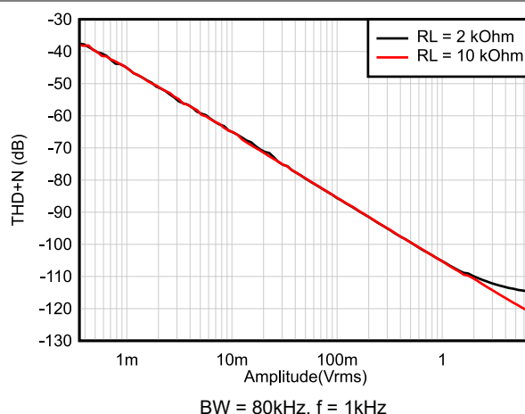
FIG 5-20. THD+N vs Output Amplitude
