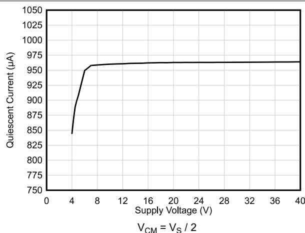
FIG 5-21. Quiescent Current vs Supply Voltage
