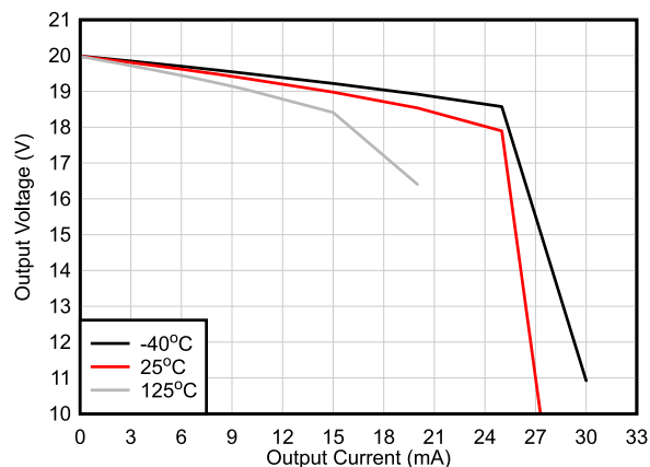
図 5-12. Output Voltage Swing vs Output Current (Sourcing)
