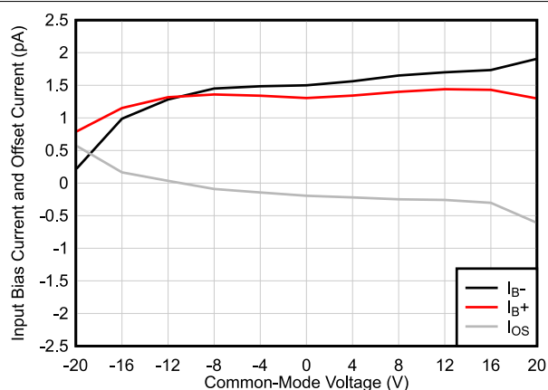
図 5-10. Input Bias Current vs Common-Mode Voltage
