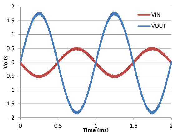
図 9-2. Input and Output Voltages of the Inverting Amplifier
