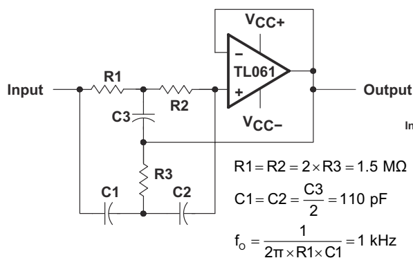
図 9-5. High-Q Notch Filter
