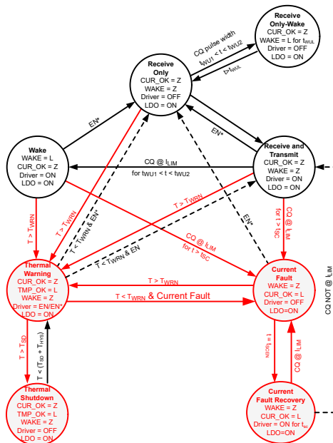
☒ 8-3. Device State Diagram
