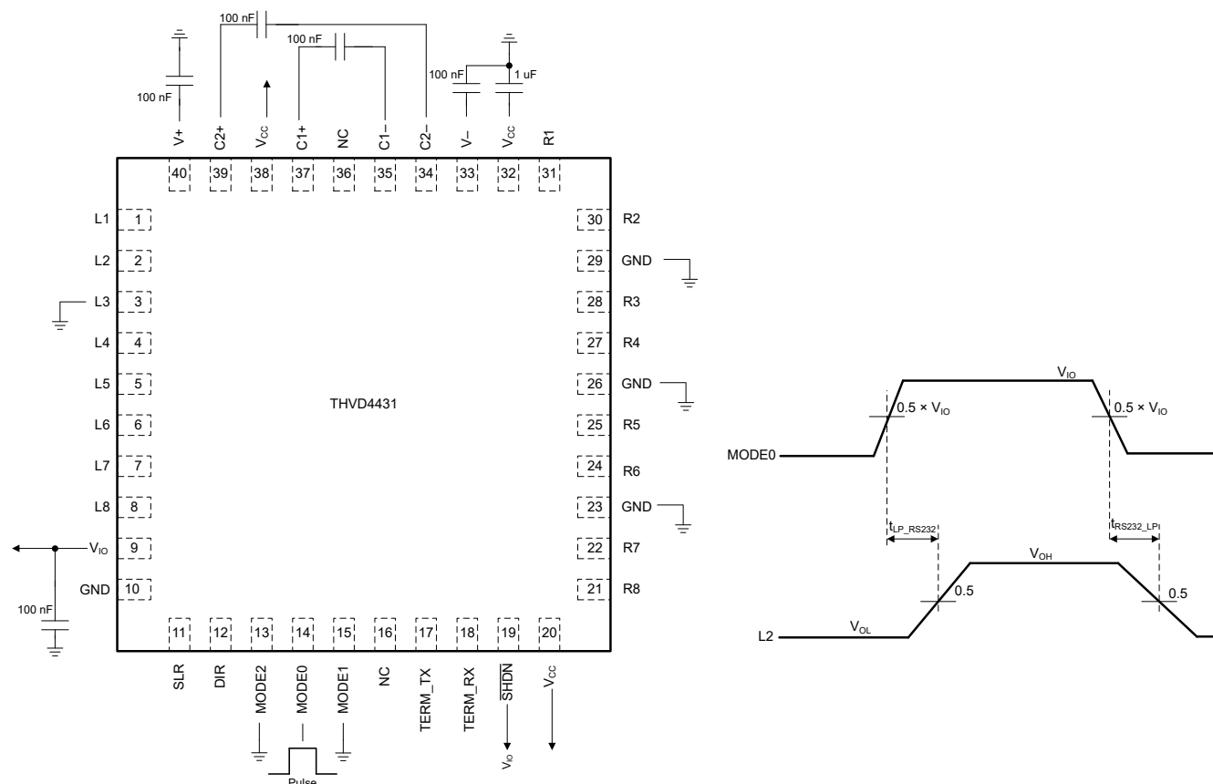
図 6-13. Time to Switch from RS-232 Loopback to Normal RS-232 3T5R Mode and Back
