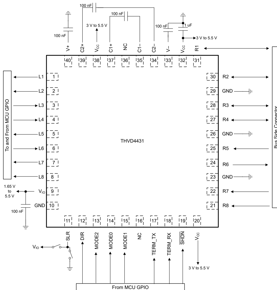
8-5. Typical application diagram for THVD4431
