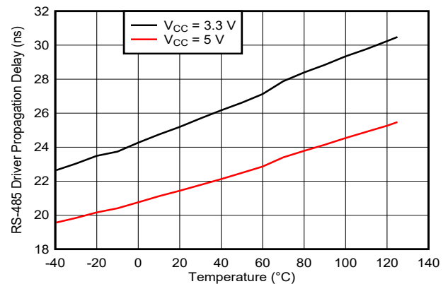
FIG 5-12. RS-485 20Mbps Driver Propagation Delay vs Temperature
