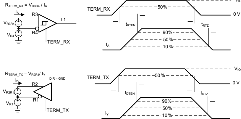
図 6-10. Termination Resistor Switching Measurement
