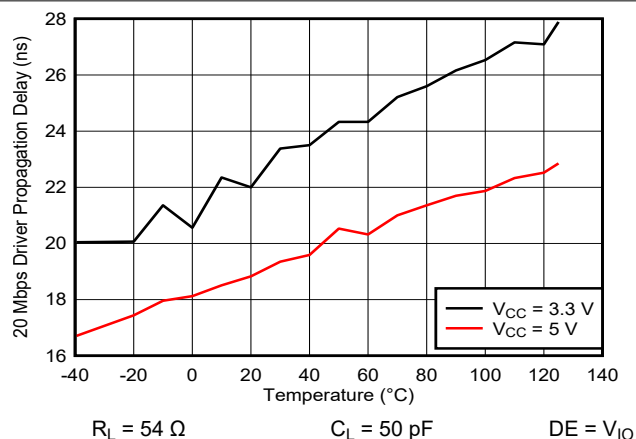
FIG 6-8. Driver Propagation Delay vs Temperature (20 Mbps)
