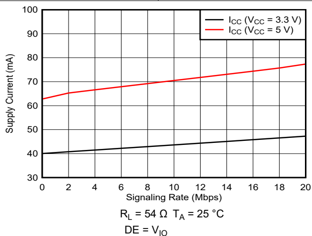
FIG 6-9. Supply Current vs Signal Rate (20 Mbps)
