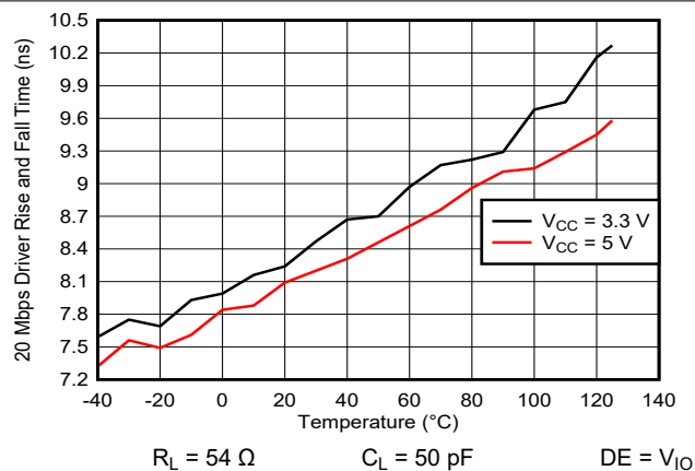
FIG 6-7. Driver Rise or Fall Time vs Temperature (20 Mbps)
