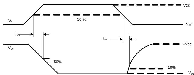
FIG 24. Measurement of Driver Enable and Disable Times With Active Low Output and Pull-up Load
