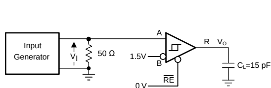
FIG 25. Measurement of Receiver Output Rise and Fall Times and Propagation Delays
