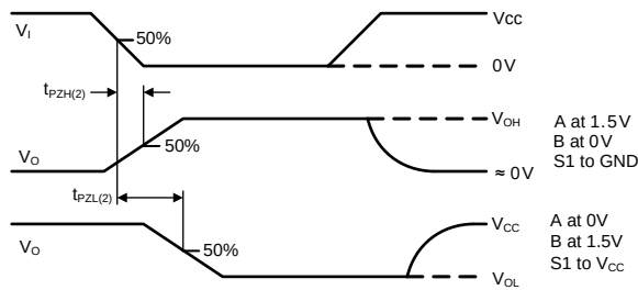
FIG 27. Measurement of Receiver Enable Times With Driver Disabled
