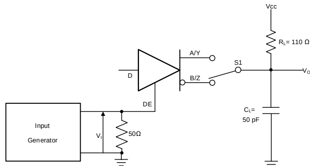
FIG 24. Measurement of Driver Enable and Disable Times With Active Low Output and Pull-up Load
