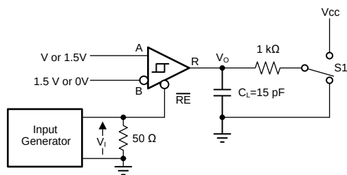
FIG 27. Measurement of Receiver Enable Times With Driver Disabled
