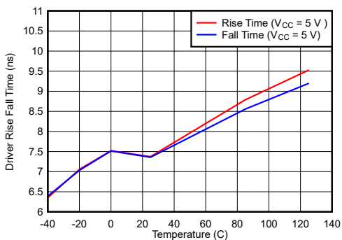
6-7. Driver Rise or Fall Time vs Temperature (THVD1426)
