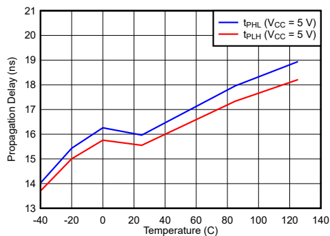
6-8. Driver Propagation Delay vs Temperature (THVD1426)
