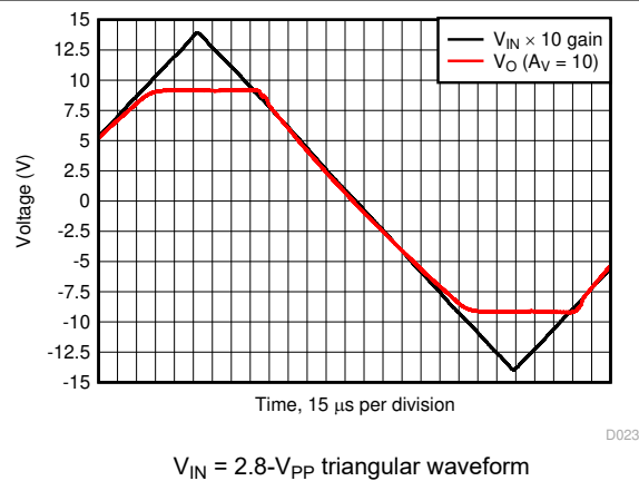
図 5-24. Overdrive Recovery
