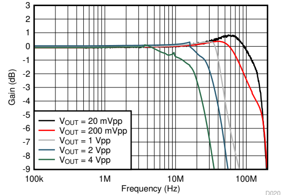
Figure 6-20. Frequency Response vs V_{\text{OUT}}
