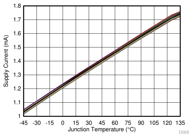
図 10-1. Linear Temperature Coefficient for Supply Current
