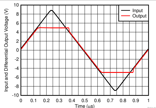
Figure 6-12. Overdrive Recovery Performance
