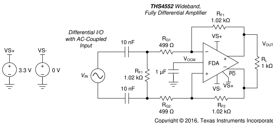
FIG 8-10. Example AC-Coupled Differential Input Design
