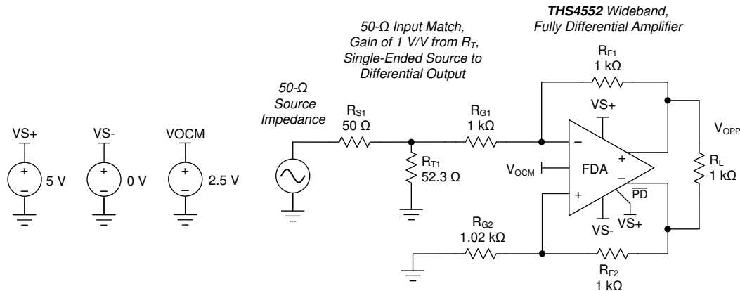
图 8-9. DC-Coupled Gain of 1 with R_F = 1 \text{ k}\Omega and Single-to-Differential Matched Input 50 Ω Impedance
