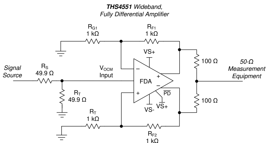
Figure 8-5. Output Common-Mode Measurements
