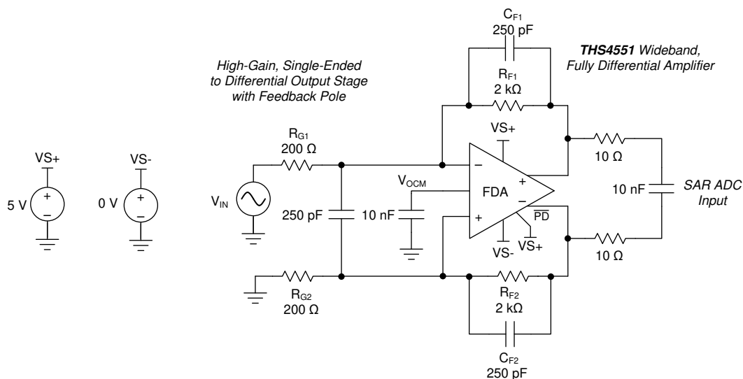
10-9. Single-Ended to Differential Stage with a Feedback Pole and Differential Input Capacitor
