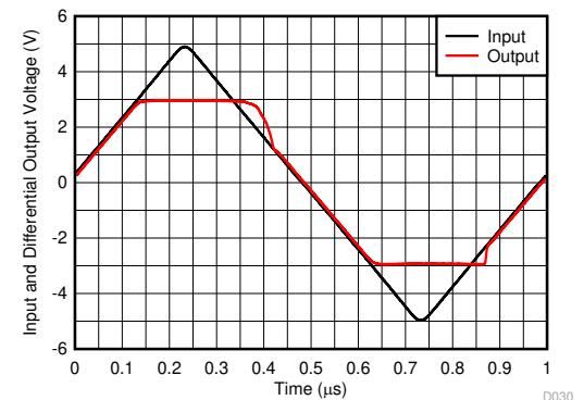
Figure 7-30. Overdrive Recovery Performance
