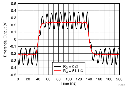
Figure 7-28. Step Response Into Capacitive Load
