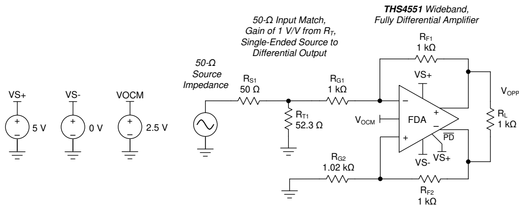
图 9-9. DC-Coupled Gain of 1 with R_F = 1 \text{ k}\Omega and Single-to-Differential Matched Input 50-Ω Impedance
