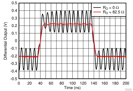
Figure 7-26. Step Response Into Capacitive Load
