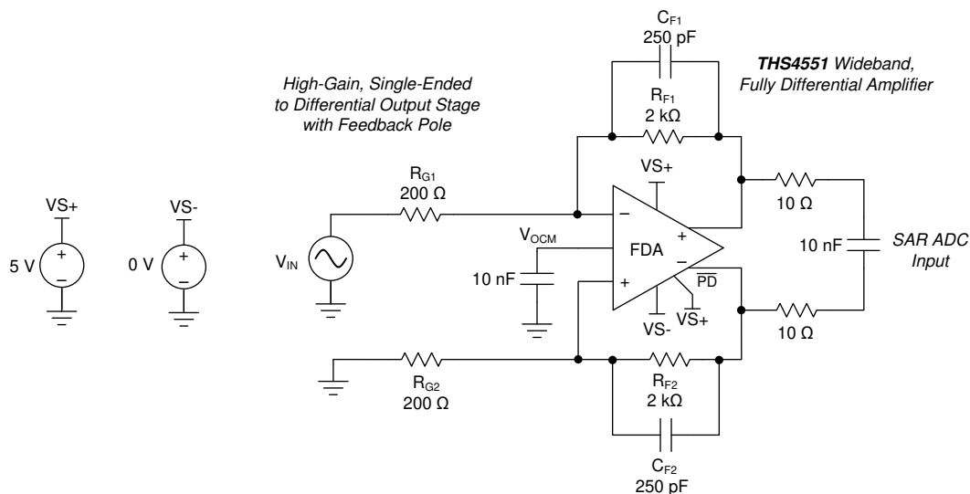
10-7. Single-Ended to Differential Stage with a Feedback Pole
