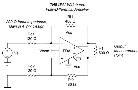
8-1. 200- \Omega Input Impedance, Single-Ended to Differential DC-Coupled Design with Gain of 4 V/V
