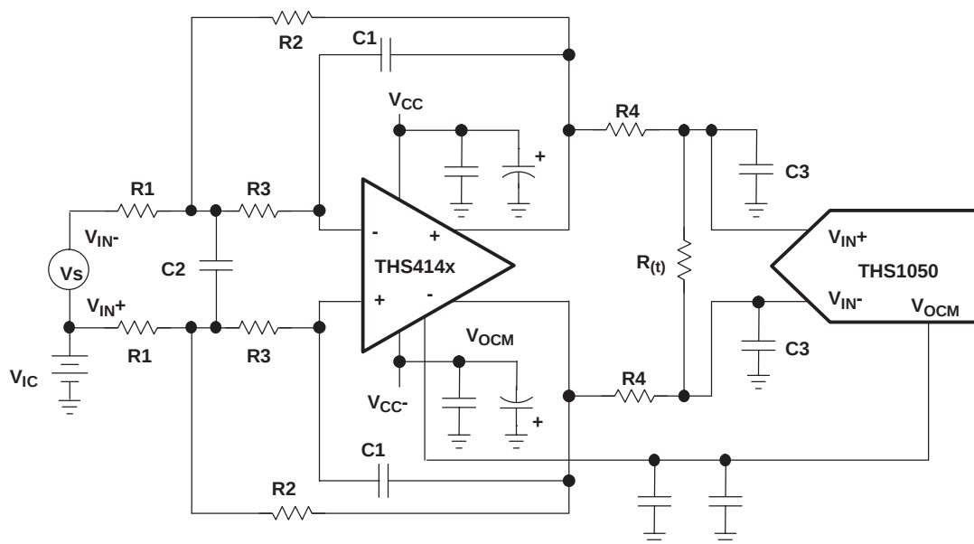
Figure 26. Antialias Filtering
