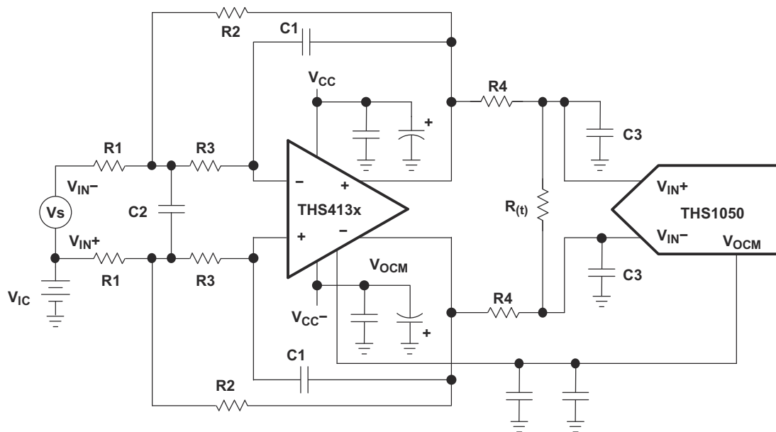
図 9-5. Antialias Filtering
