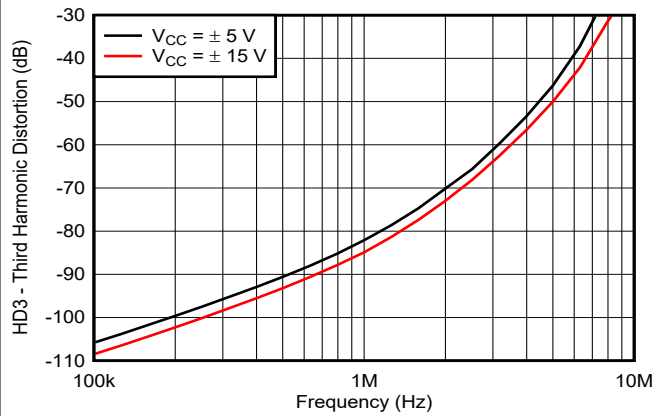
FIG 7-20. Third-Harmonic Distortion vs Frequency
