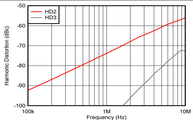
FIG 5-14. Harmonic Distortion vs Frequency
