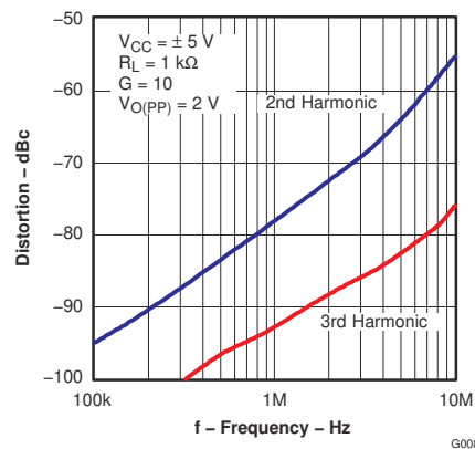
Figure 5-37. Distortion vs Frequency
