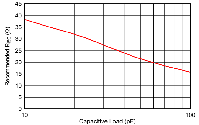
Gain = 5 V/V, R_F = 1\text{ k}\Omega 7-8. Recommended R_{ISO} vs Capacitive Load
