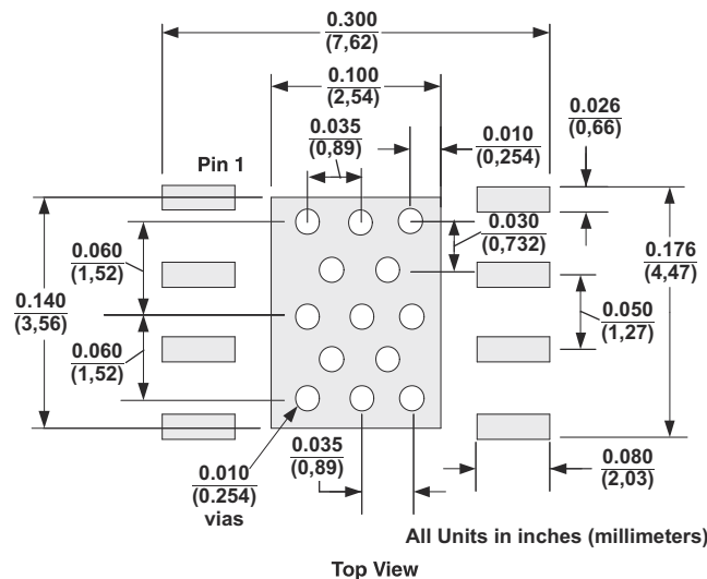
☒ 9-7. DDA PowerPAD PCB Etch and Via Pattern
