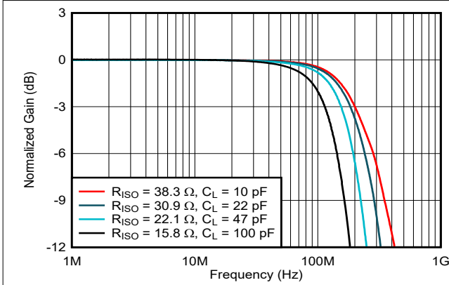
V_{OUT} = 200\text{ mV}_{PP} , Gain = 5 V/V, R_F = 1\text{ k}\Omega 7-7. Capacitive Load Frequency Response
