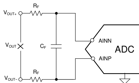
Figure 9-9. Differential Filter
