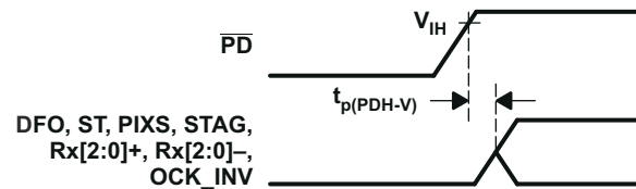
FIG 6-8. Delay From \overline{\text{PD}} Low to High Until Inputs Are Active
