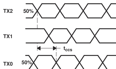
FIG 6-12. Analog Input Channel-to-Channel Skew
