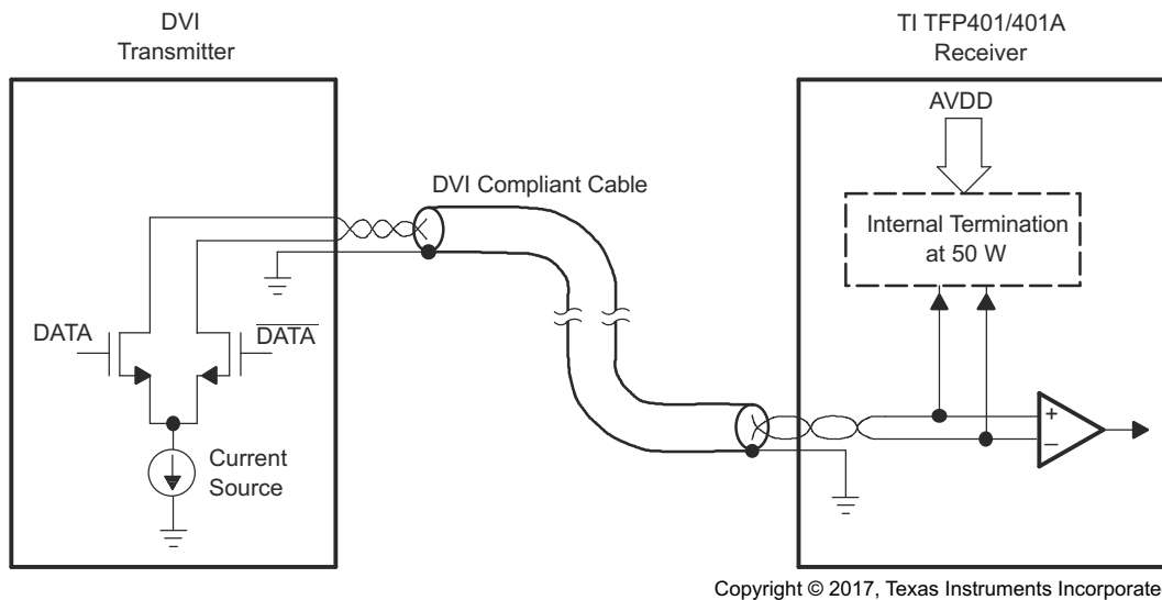
FIG 7-1. TMSD Differential Input and Transmitter Connection
