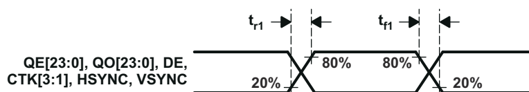
FIG 6-1. Rise and Fall Times of Data and Control Signals
