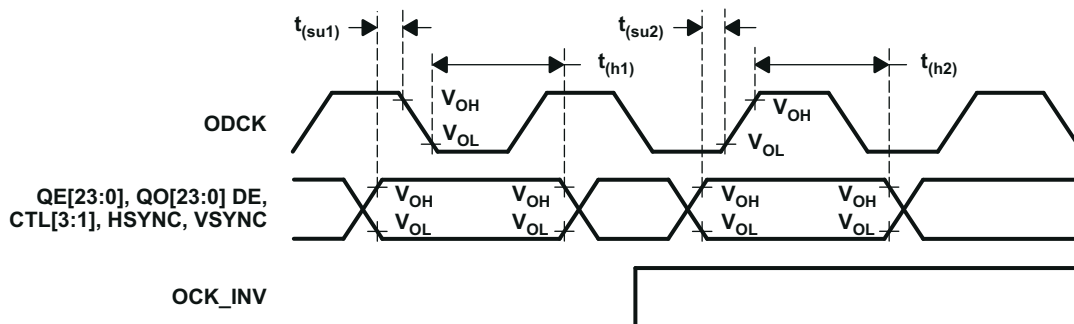
图 6-4. Data Setup and Hold Times to Rising and Falling Edges of ODCCK
