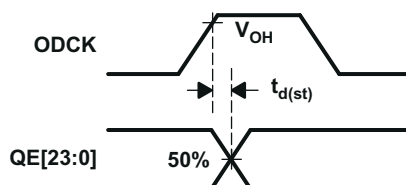
图 6-5. ODCCK High to QE[23:0] Staggered Data Output
