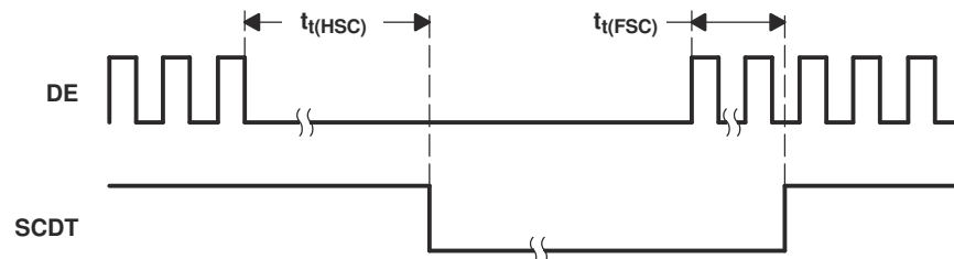
FIG 6-9. Time From DE Transitions to SCDT Low and SCDT High
