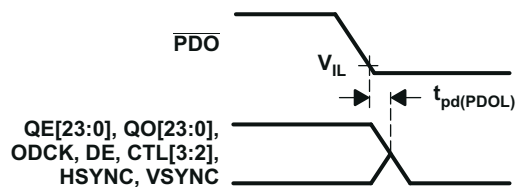
图 6-7. Delay From \overline{PDO} Low to Hi-Z Outputs
