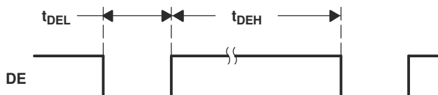
6-13. Minimum DE Low and Maximum DE High
