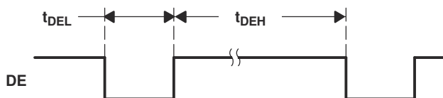
✎ 8-13. Minimum DE Low and Maximum DE High
