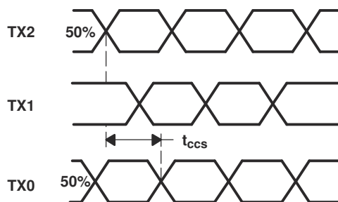
✎ 8-11. Analog Input Channel-to-Channel Skew
