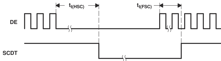
✎ 8-12. Time Between DE Transitions to SCDT Low and SCDT High
