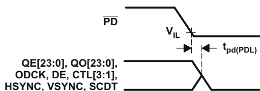
8-7. Delay From \overline{\text{PD}} Low to Hi-Z Outputs
