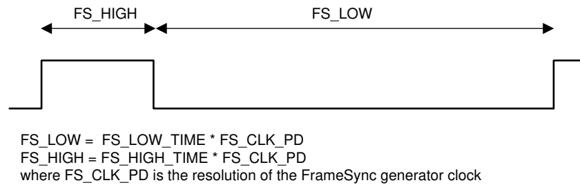
図 7-17. Internal FrameSync Signal
