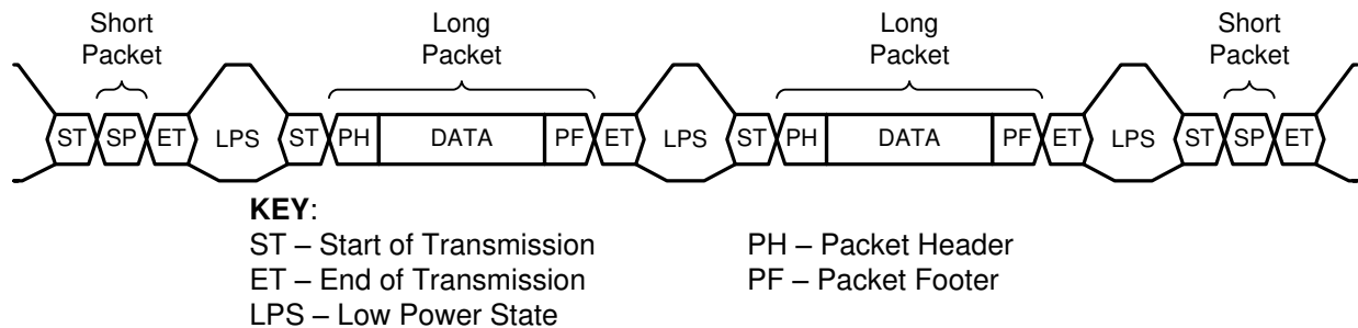
図 7-6. CSI-2 Protocol Layer With Short and Long Packets
