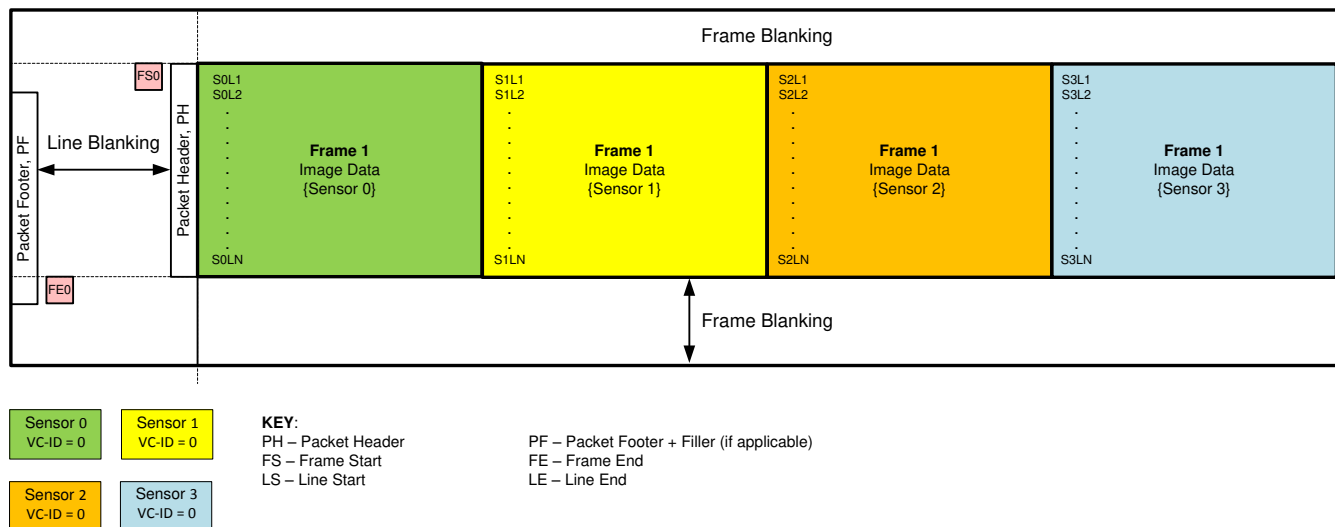
图 7-20. Line-Concatenated Format
