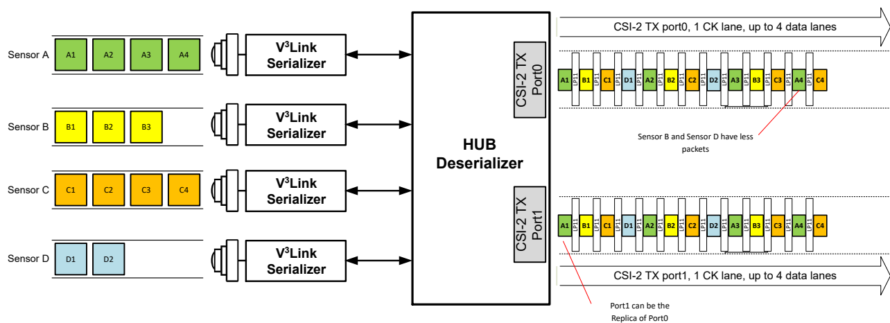
図 7-14. Four Sensor Data onto 1xCSI-2 Replicated With Virtual Channels (VC-ID) With Different Frame Size
