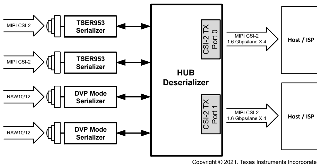
図 8-17. Two DVP Mode Serializers and Two TSER953 Sensor Data Onto CSI-2 Over 2 Ports
