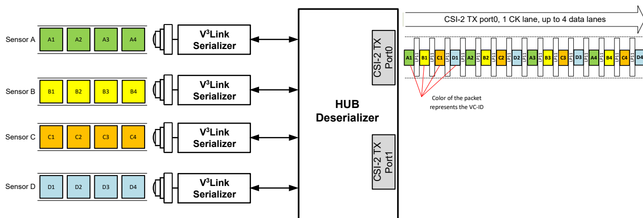
図 7-12. Four Sensor Data onto CSI-2 With Virtual Channels (VC-ID)
