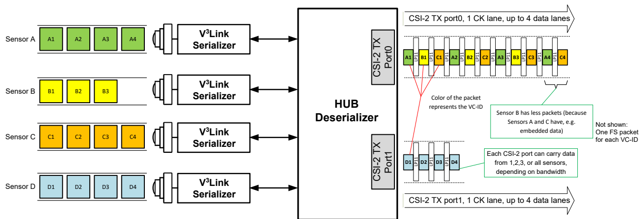
図 7-13. Four Sensor Data onto CSI-2 With Virtual Channels (VC-ID) With Different Frame Size
