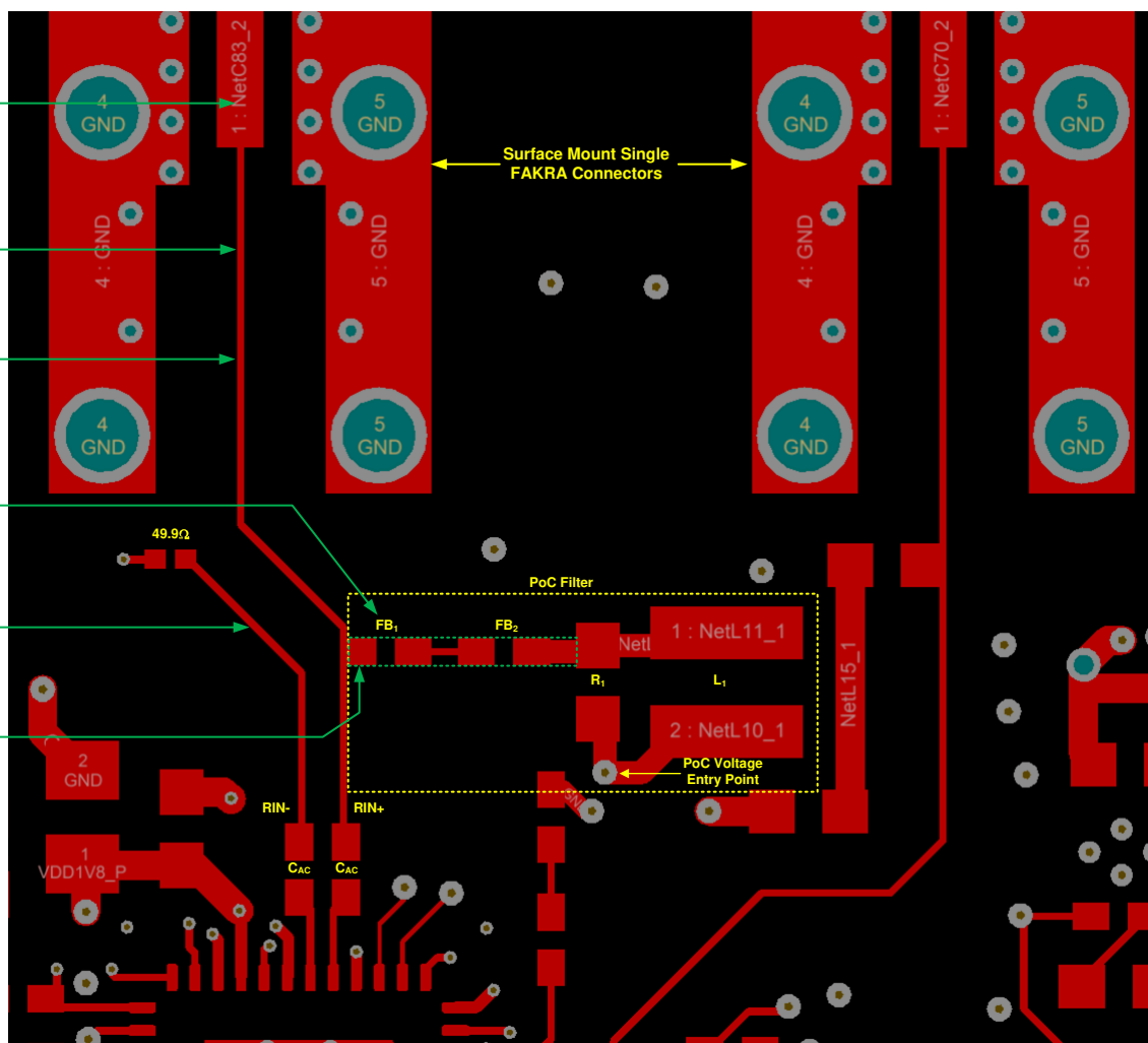
8-22. Example Routing of V³Link Traces to a Single Mini-Fakra Connector and PoC Components
