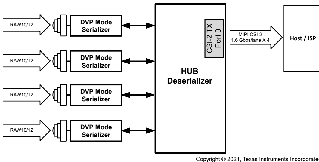
図 8-14. Four DVP Mode Serializers Sensor Data Onto CSI-2 Over 1 Port
