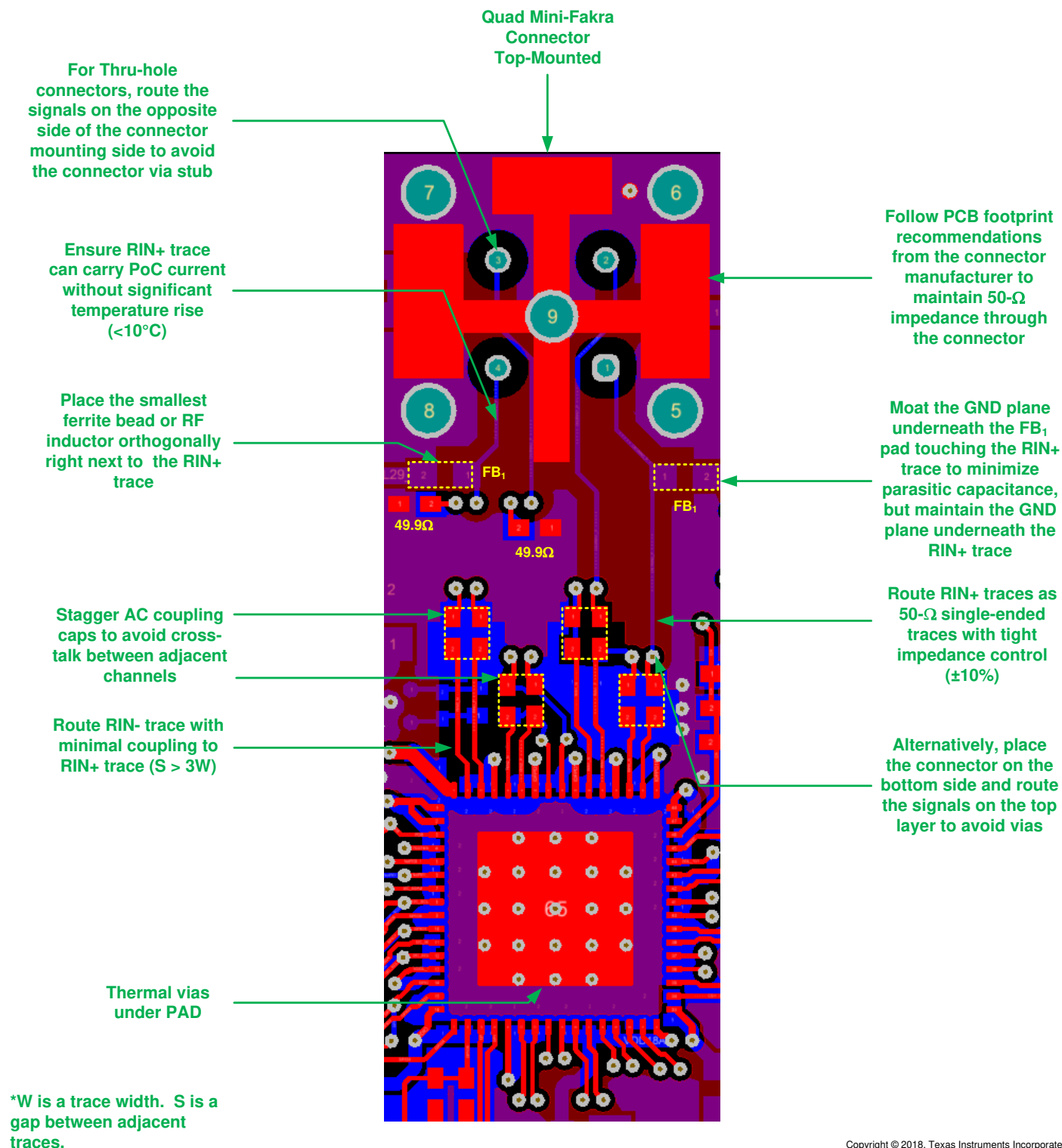
✎ 8-21. TDES960 Example PCB Layout With Quad Mini-Fakra Connector
