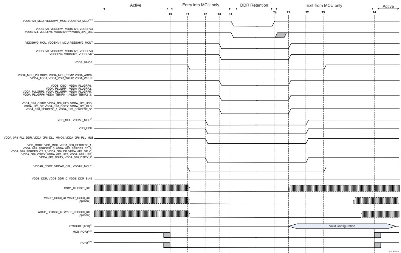
☒ 6-8. Entry and Exit of DDR Retention Sequencing
