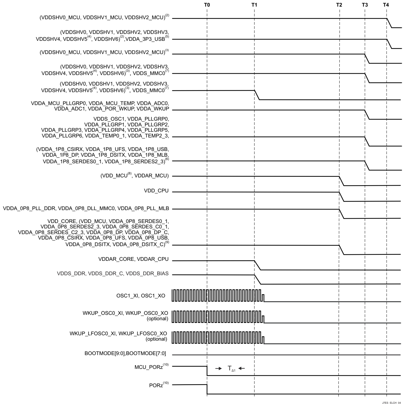
6-6. Isolated MCU and Main Domains, Primary Power- Down Sequencing
