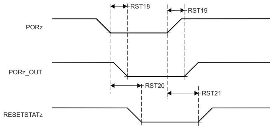
図 6-12. PORz initiates; PORz_OUT and RESETSTATz Switching Characteristics
