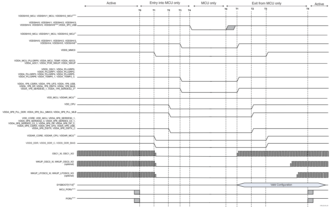
図 6-7. Entry and Exit of MCU Only Sequencing
