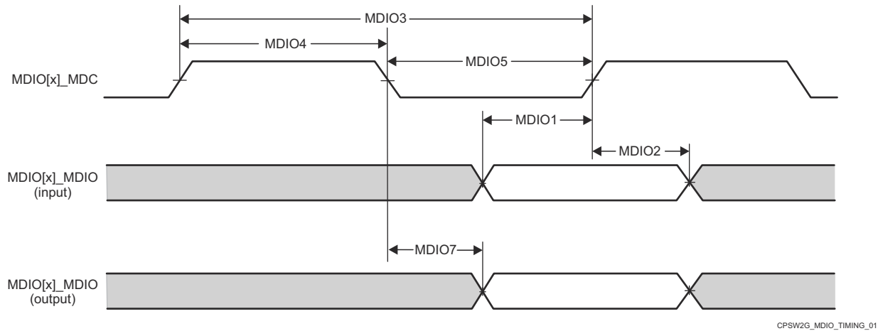
図 6-41. CPSW2G MDIO Timing Requirements and Switching Characteristics
