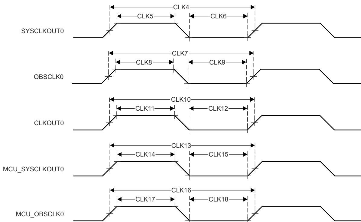
6-21. Clock Switching Characteristics
