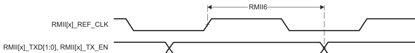
図 6-44. RMII[x]_TXD[1:0], and RMII[x]_TX_EN Switching Characteristics – RMII Mode
