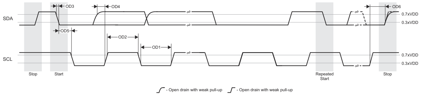
図 6-81. I3C Open Drain Timing Requirements
