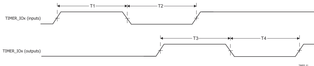
図 6-119. Timer Timing
