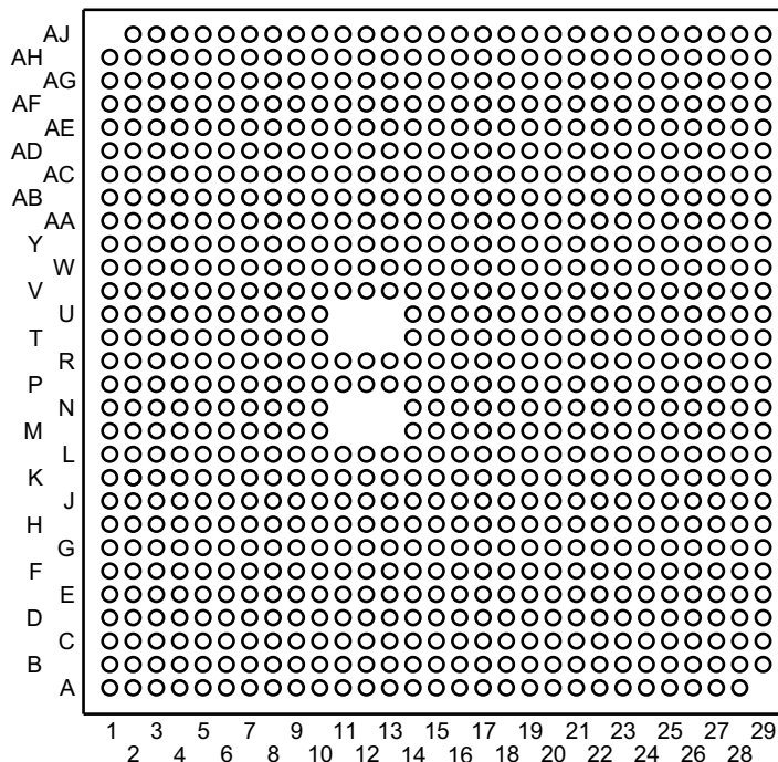
図 5-1. ALF FCBGA-N827 Pin Diagram (Bottom View)
