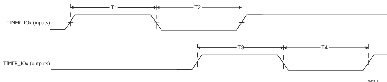
図 6-119. Timer Timing
