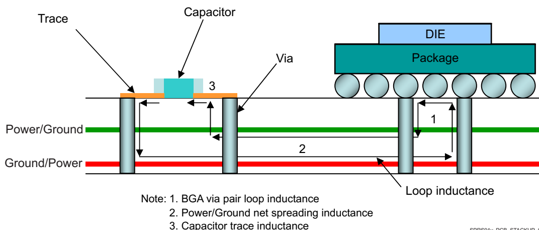
FIG 8-1. Minimize Loop Inductance With Proper Layer Assignment
