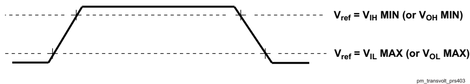
7-3. Rise and Fall Transition Time Voltage Reference Levels
