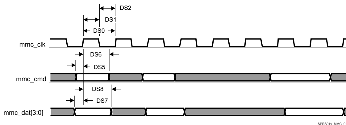
图 7-39. MMC/SD/SDIOj in - Default Speed - Receiver Mode
