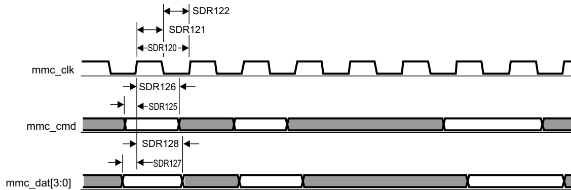
图 7-43. MMC/SD/SDIOj in - SDR12 - Receiver Mode
