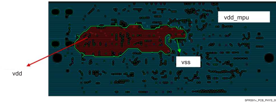
8-2. Coplanar Shielding of Power Net Using Ground Guard-band
