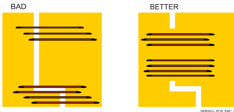
8-11. Trace Examples
