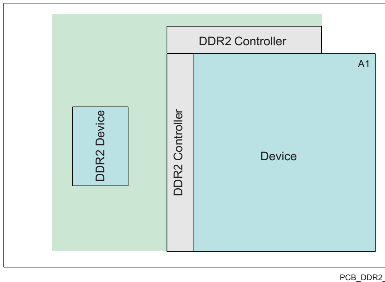
8-41. DDR2 Keepout Region
