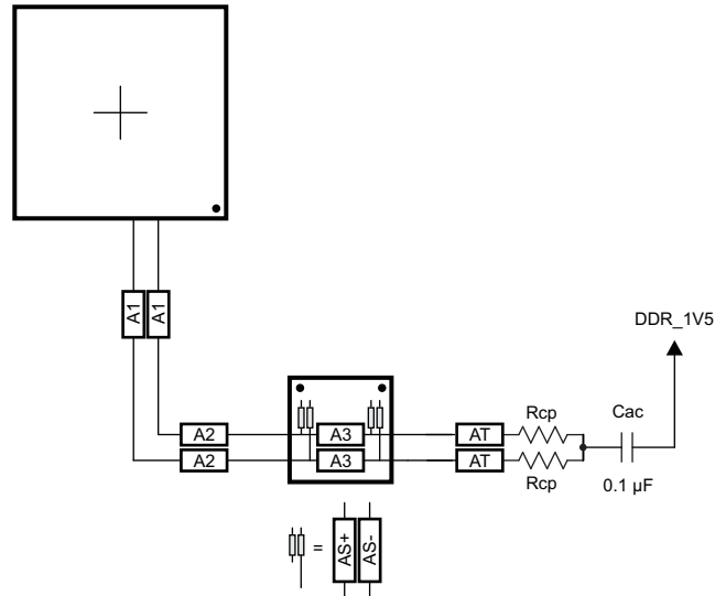
8-53. CK Routing for Two Mirrored DDR3 Devices
