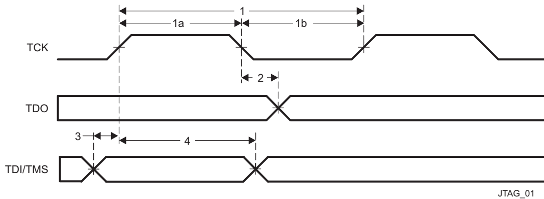
图 5-101. JTAG Timing
