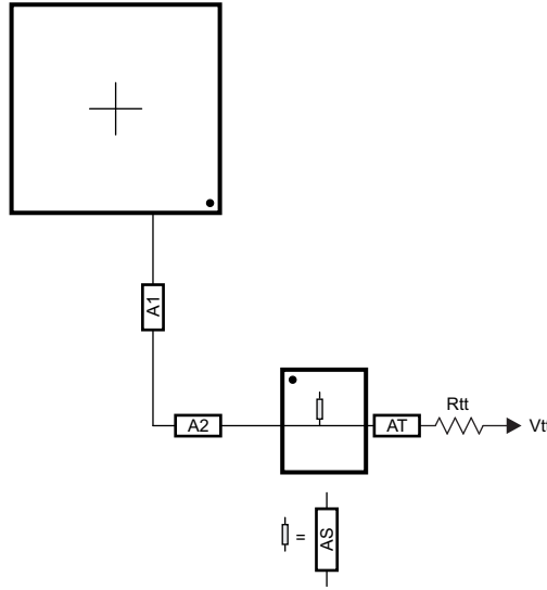
SPRS906_PCB_DDR3_21
