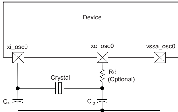
Figure 5-12. Crystal Implementation
