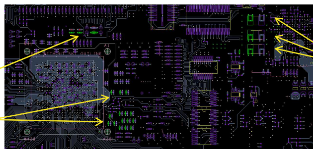
图 7-24. vdd_mpu routing and cap placements [Bottom Layer]
