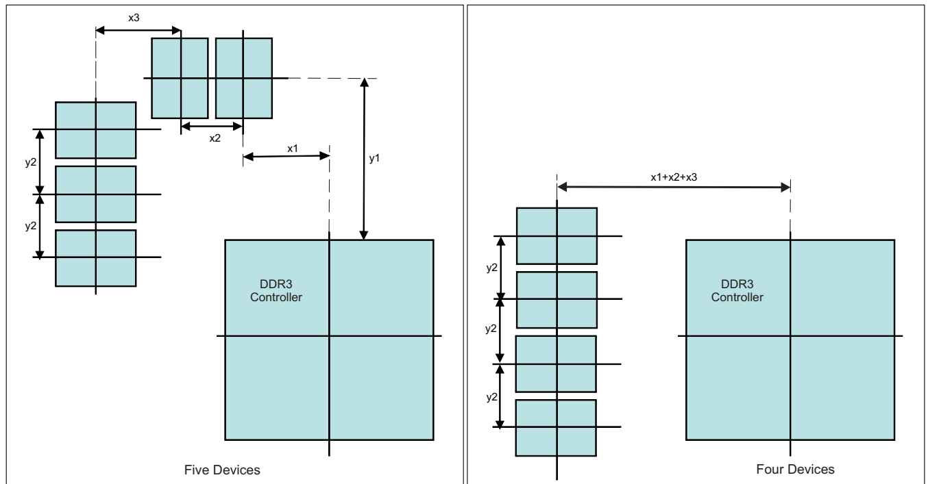
图 7-57. Placement Specifications
