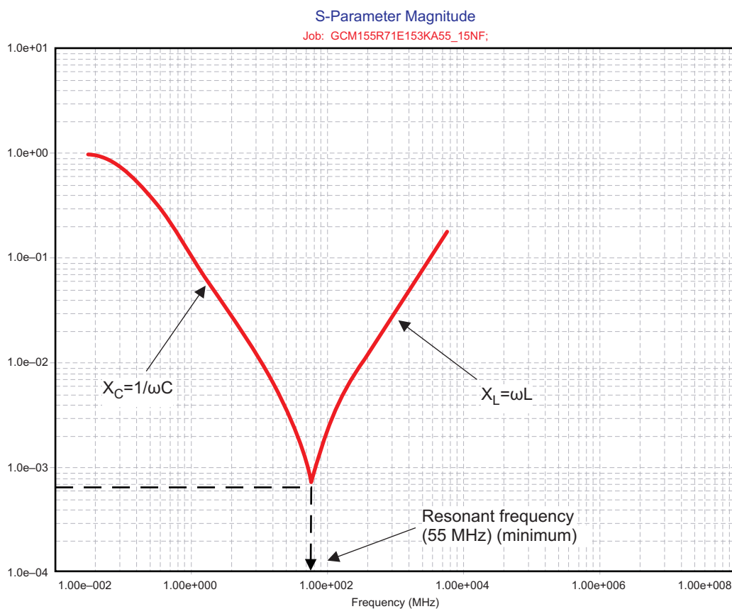
7-14. Typical Impedance Profile of a Capacitor
