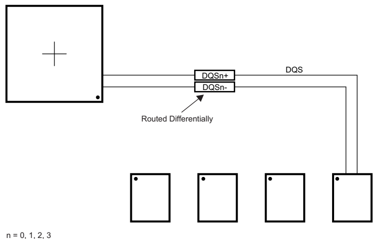
☒ 7-80. DQS Routing With Any Number of Allowed DDR3 Devices
