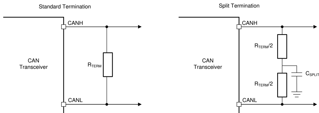
FIG 102. CAN Bus Termination Concepts
