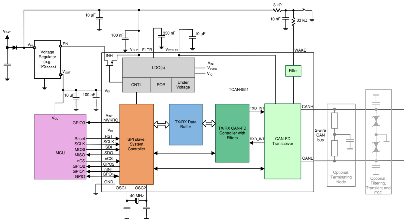
FIG 105. Typical CAN Applications for TCAN4551-Q1 for 3.3 V \mu C and Crystal
