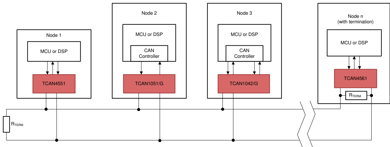
FIG 101. Typical CAN Bus
