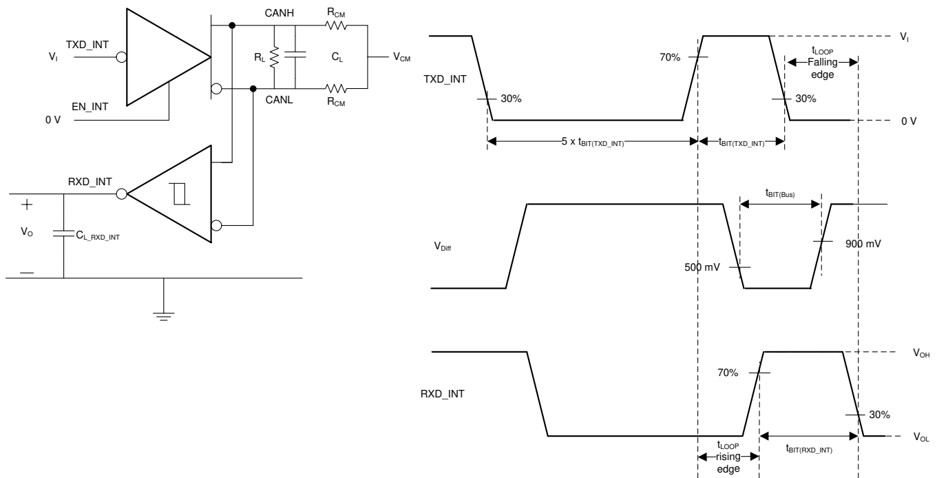
图 7. Transmitter and Receiver Timing Behavior Test Circuit and Measurement
