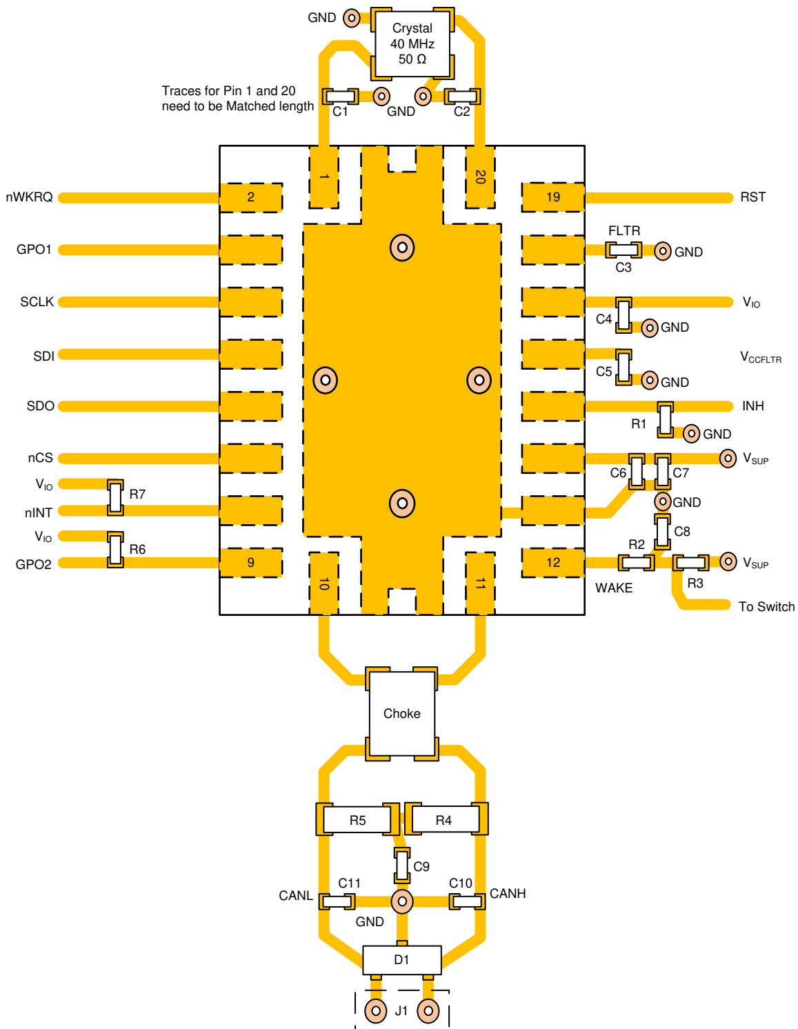
✎ 108. Example Layout
