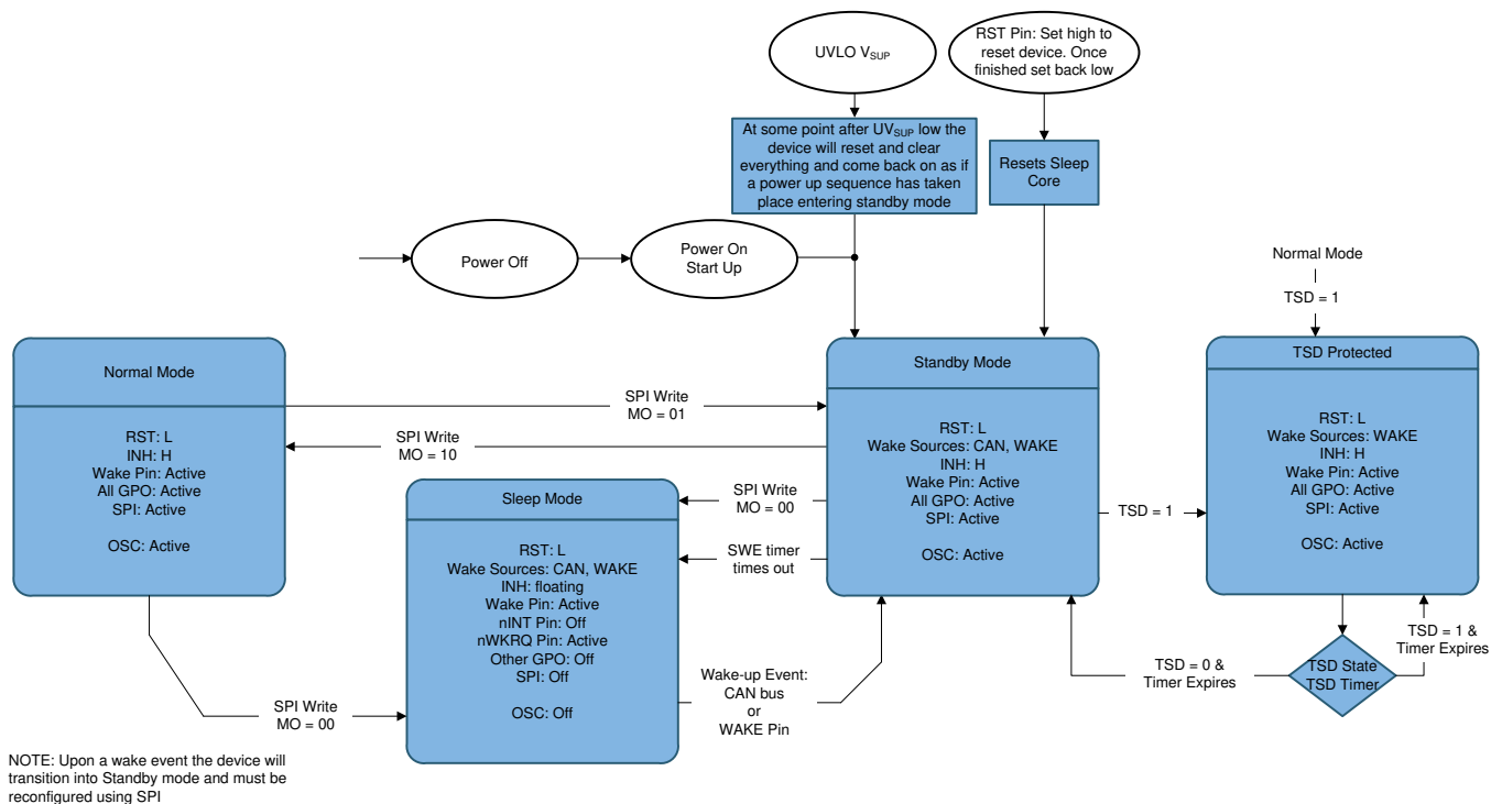
図 22. Device State Diagram
