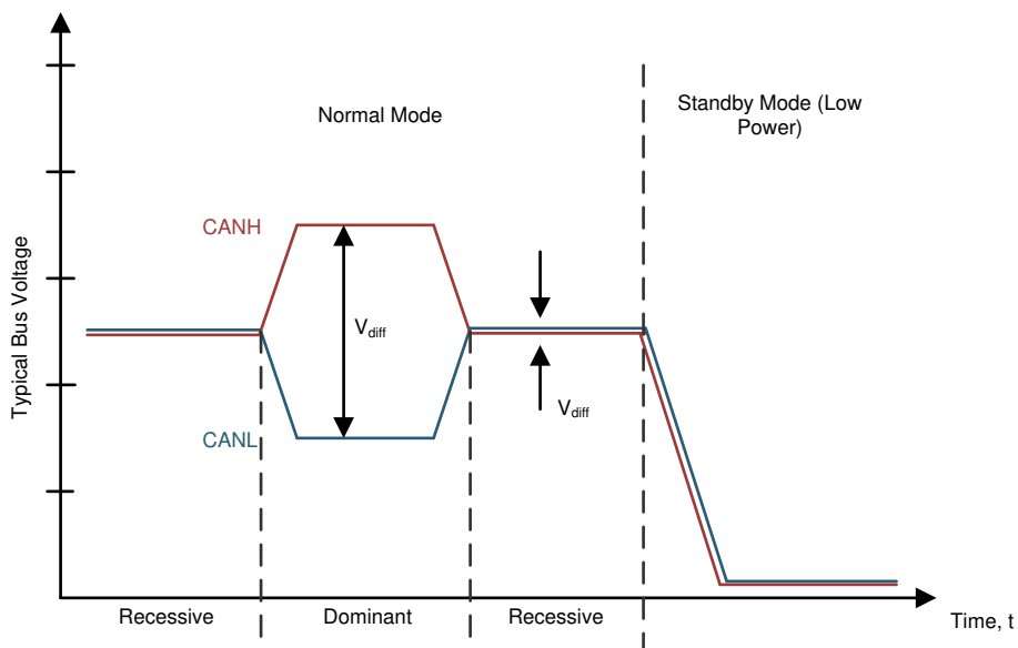
図 2. Bus States (Physical Bit Representation)
