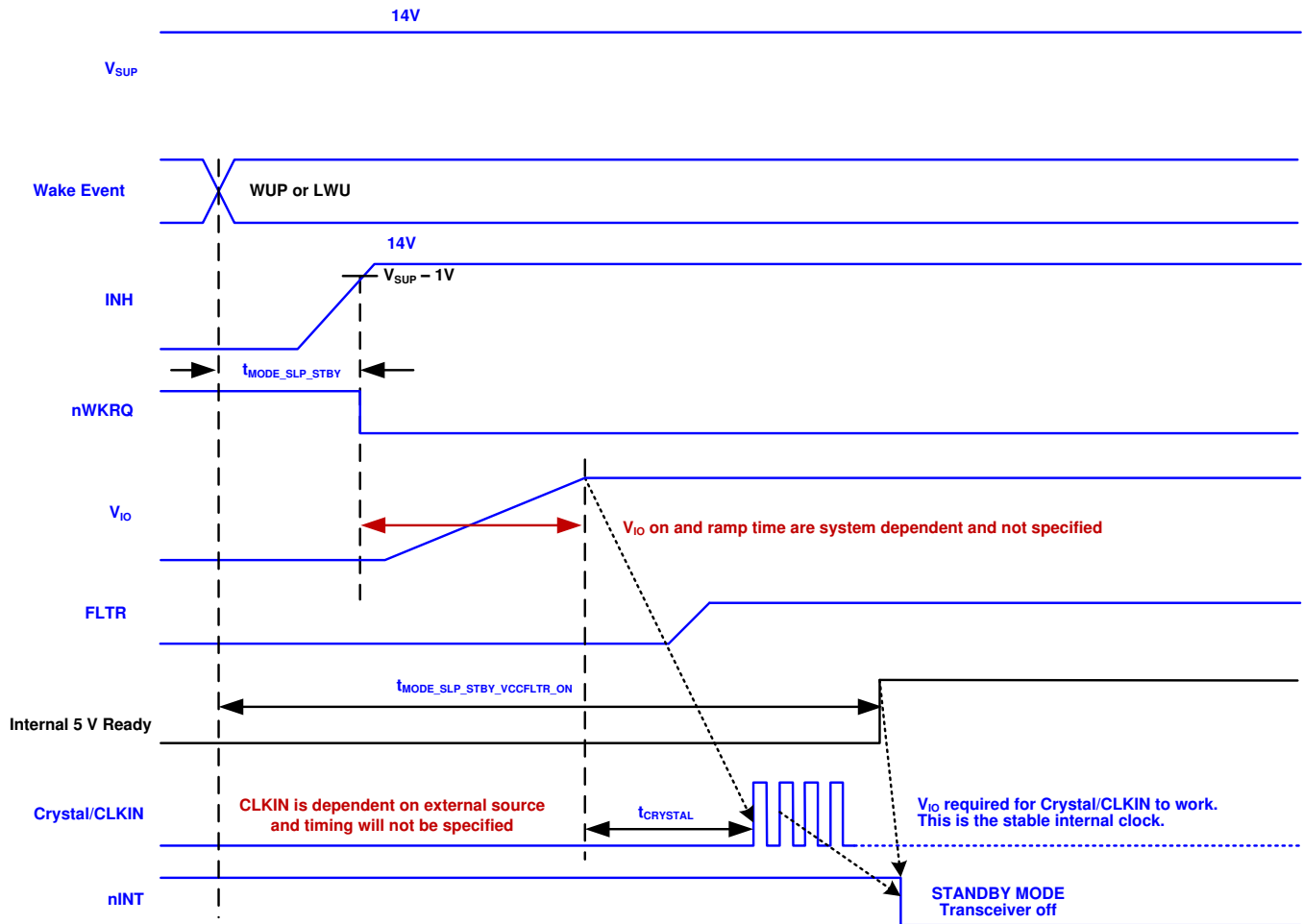
15. Sleep to Standby Timing
