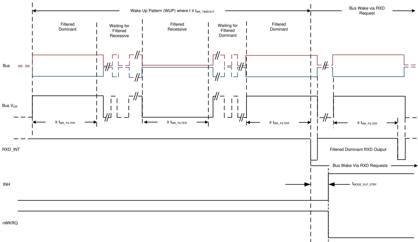
☒ 24. Wake Up Pattern (WUP) and Bus Wake via RXD_INT Request (BWRR)
