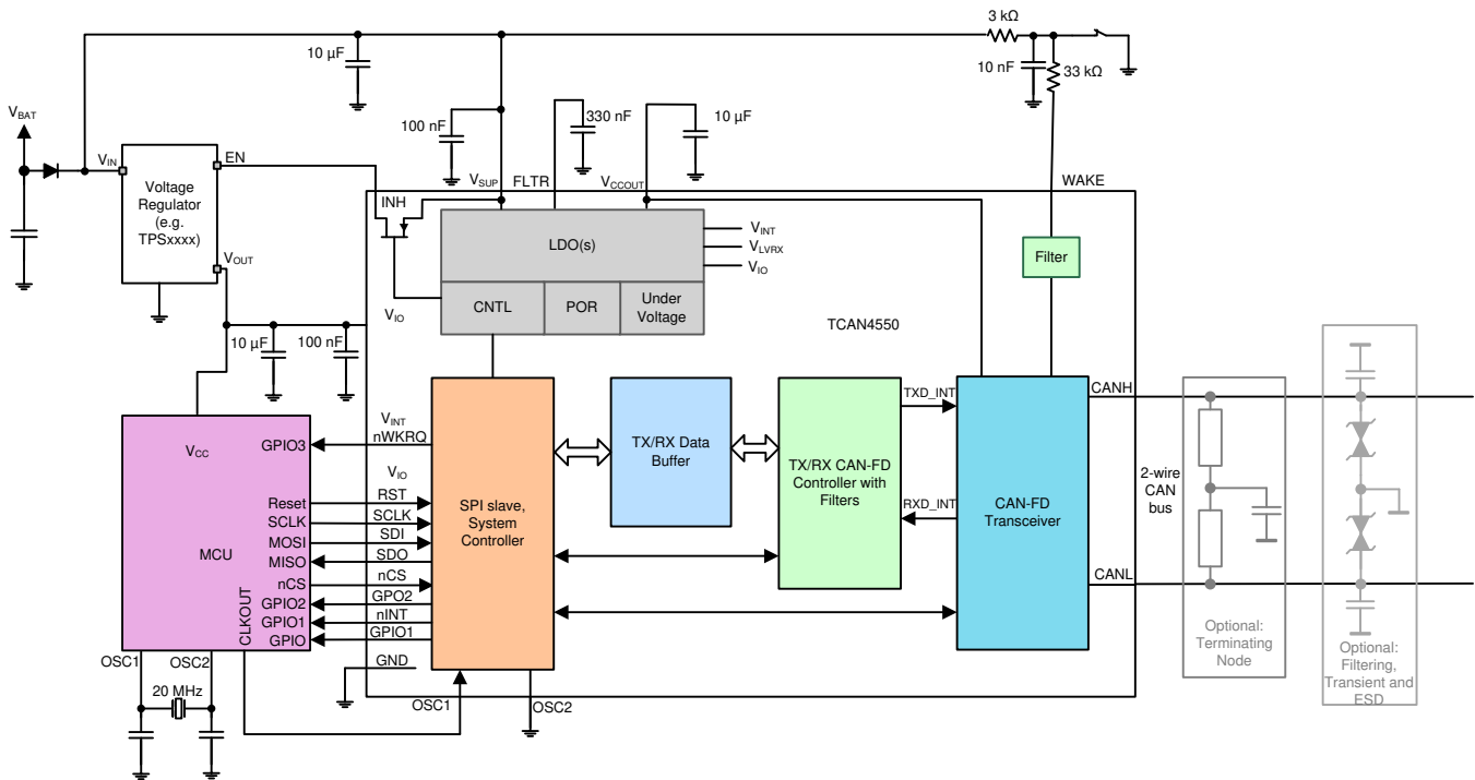
FIG 108. Typical CAN Applications for TCAN4550 for 3.3 V \mu C; Clock from MCU
