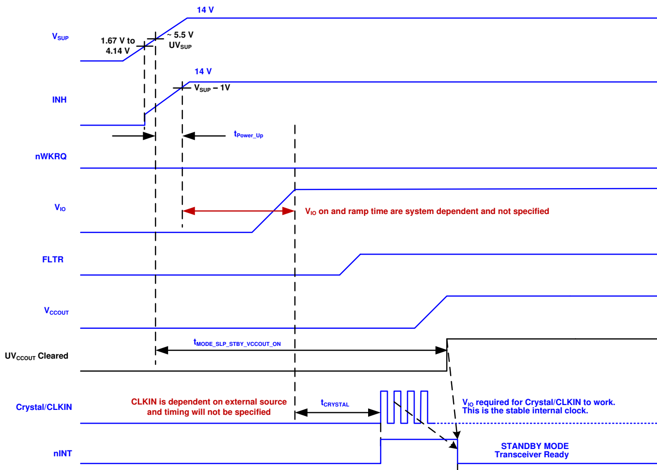
✕ 15. Power Up Timing
