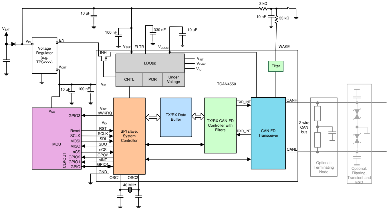
图 107. Typical CAN Applications for TCAN4550 for 3.3 V μC and Crystal
