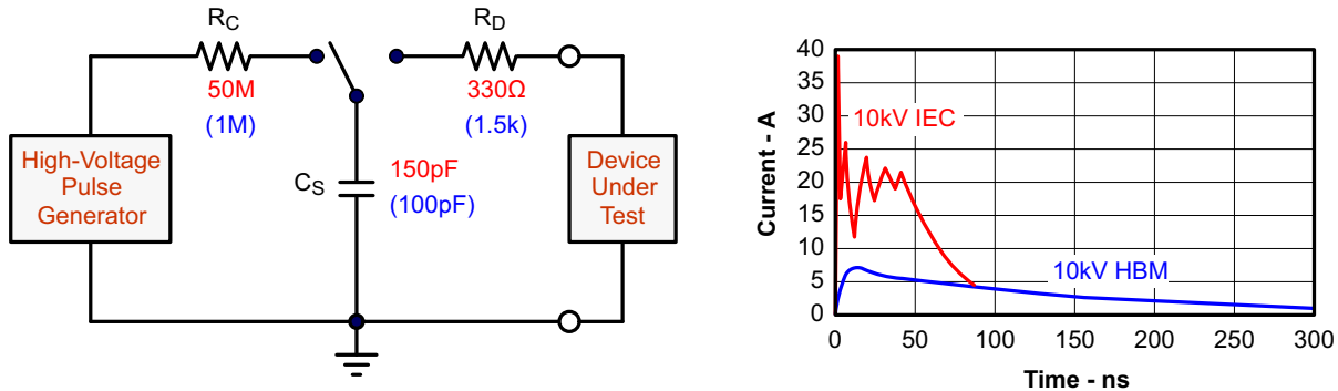
6-2. HBM and IEC-ESD Models and Currents in Comparison (HBM Values in Parenthesis)
