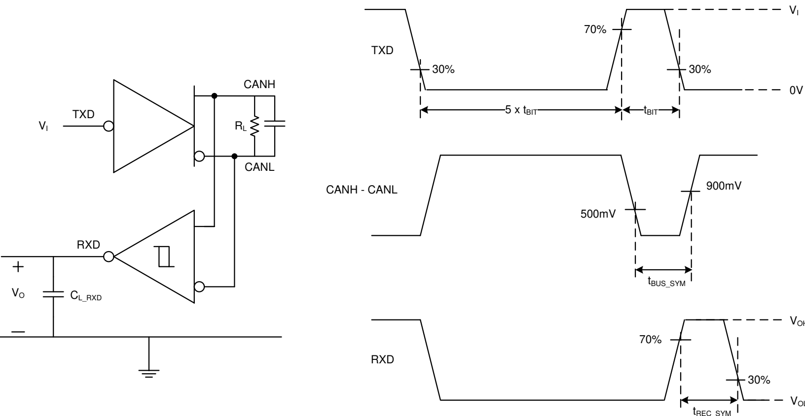
図 6-7. Loop Delay Symmetry Test Circuit and Measurement
