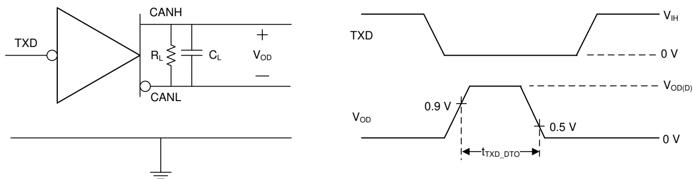
図 6-8. TXD Dominant Time Out Test Circuit and Measurement
