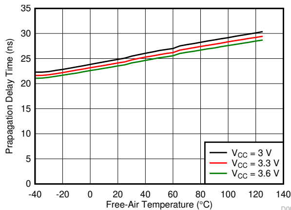
図 5-11. Driver High TXD Input to Driver Recessive Output Propagation Delay Time vs Free-Air Temperature
