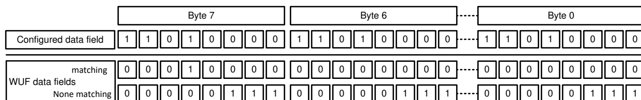
図 8-20. Data Field Validation for WUF Example
