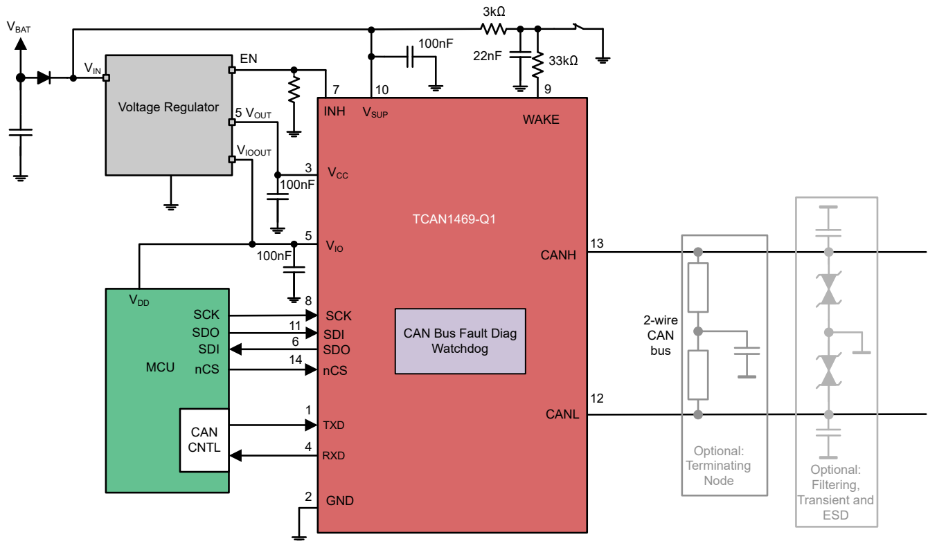
図 9-6. Typical CAN Application for TCAN1469-Q1
