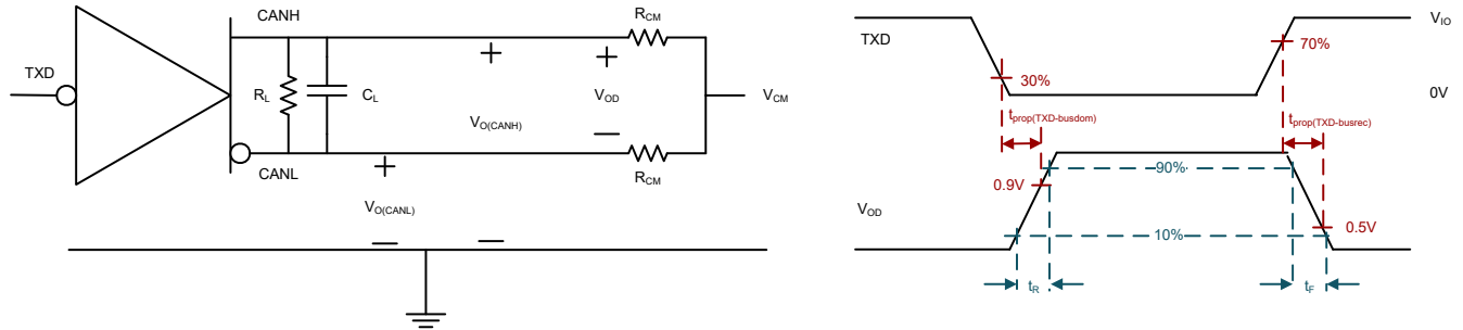
図 7-4. Driver Test Circuit and Measurement
