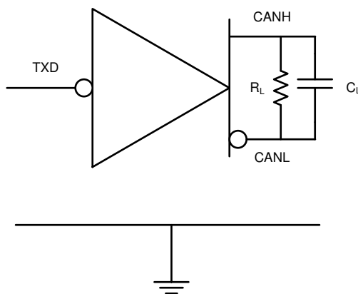
図 7-3. Supply Test Circuit
