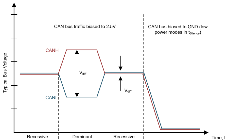
図 7-1. Bus States (Physical Bit Representation)
