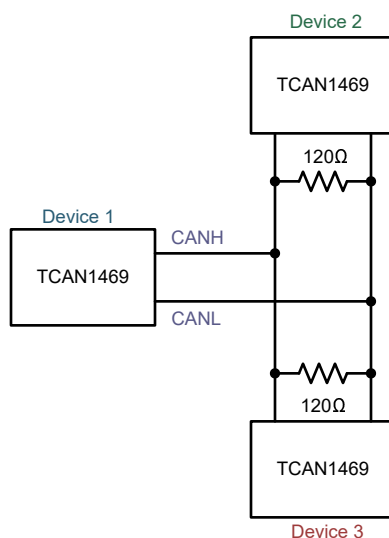
8-34. Three-Node Example
