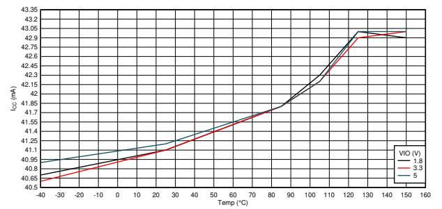
9-9. Normal Mode: I_{CC} vs Temperature Dominant
