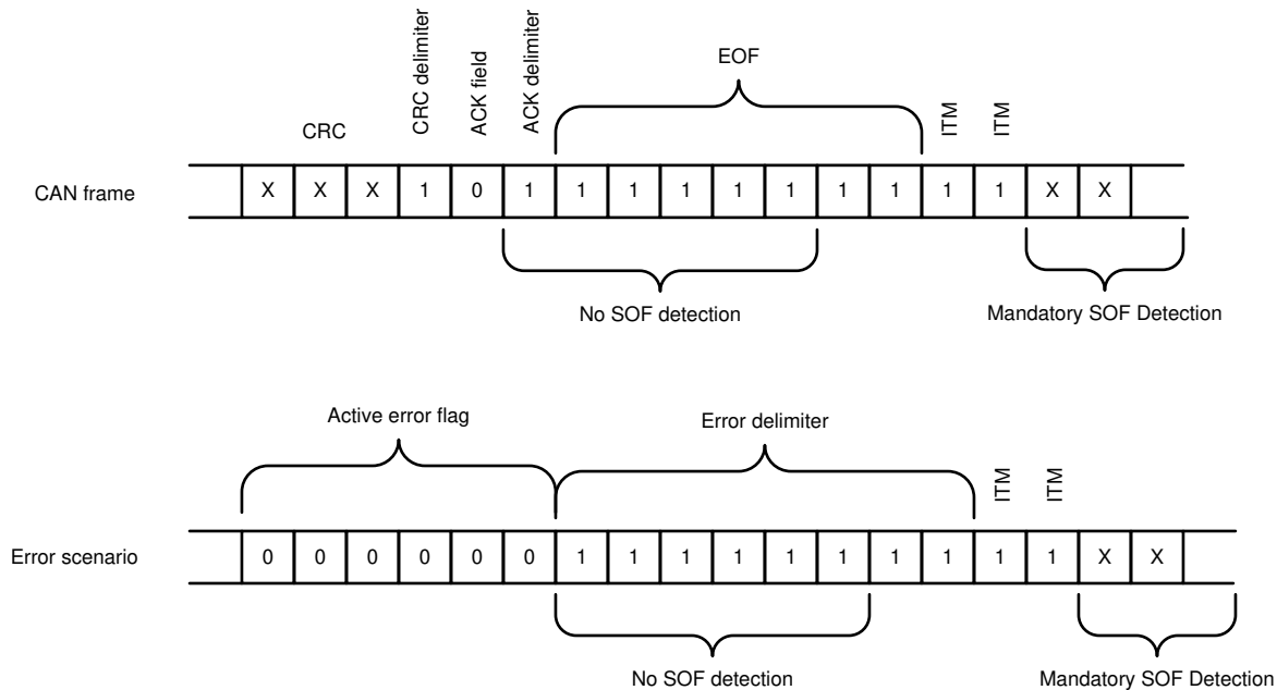
FIG 8-22. Mandatory SOF Detection after Classic CAN Frames and Error Scenarios
