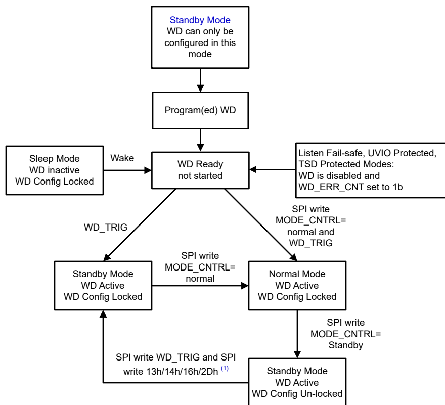
図 8-28. Watchdog Lock and Unlock Flow Chart
