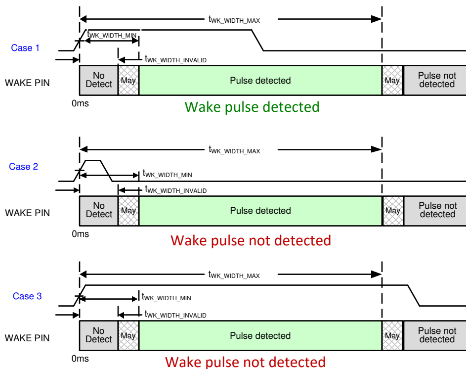
図 8-17. WAKE Pin Pulse Behavior
