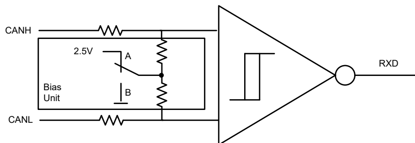
図 7-2. Simplified Recessive Common Mode Bias Unit and Receiver
