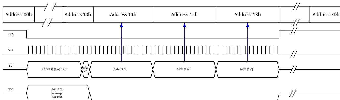
図 8-42. 32-bit SPI Burst Write
