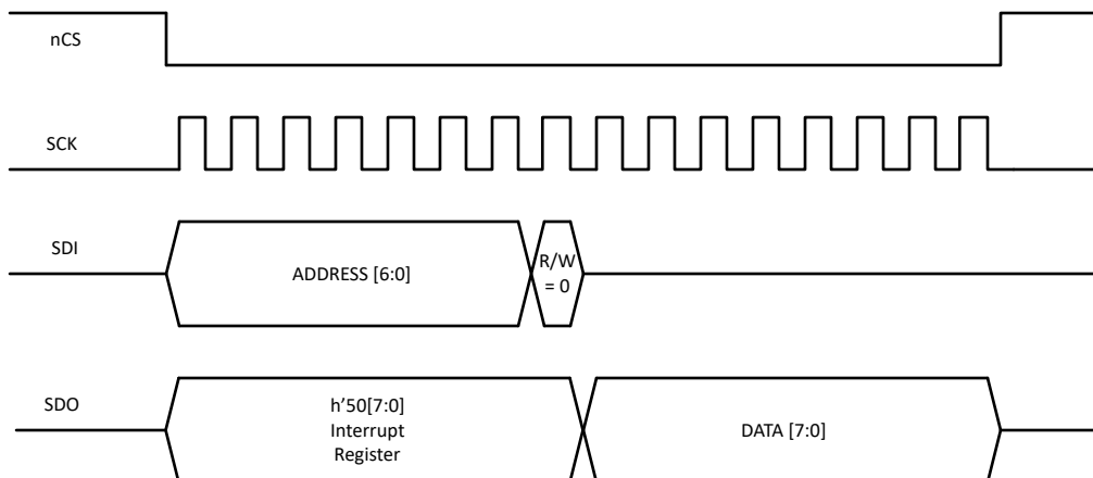
図 8-43. SPI Read
