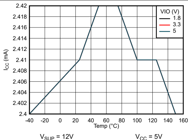
図 6-1. Normal Mode Recessive I_{CC} vs Temperature
