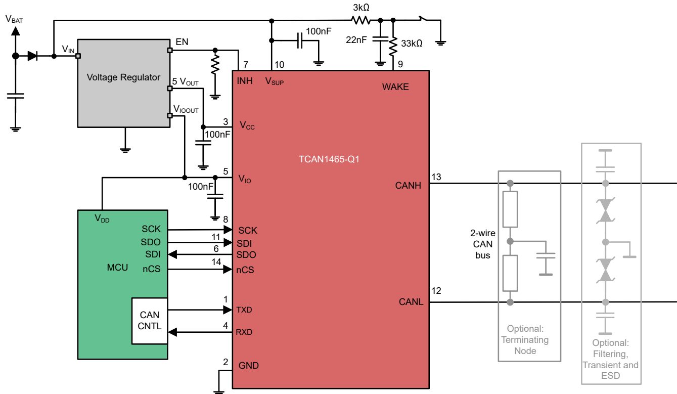
図 9-5. Typical CAN Application for TCAN1465-Q1
