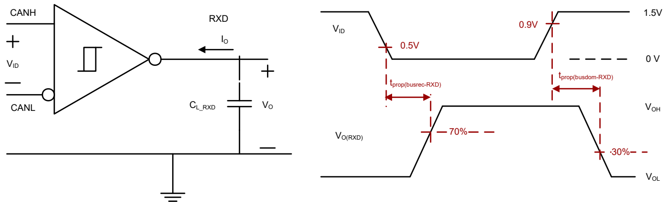
図 7-5. Receiver Test Circuit and Measurement
