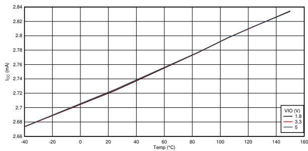
9-8. Normal Mode: I_{CC} vs Temperature Recessive
