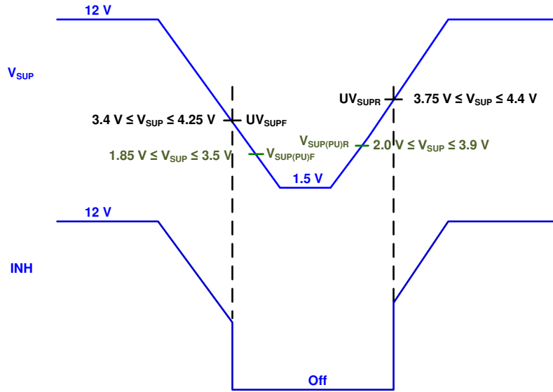
9-7. INH Behavior During Brownout
