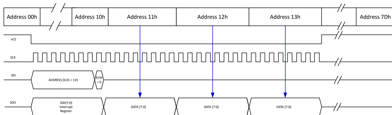
図 8-44. 32-bit SPI Burst Read
