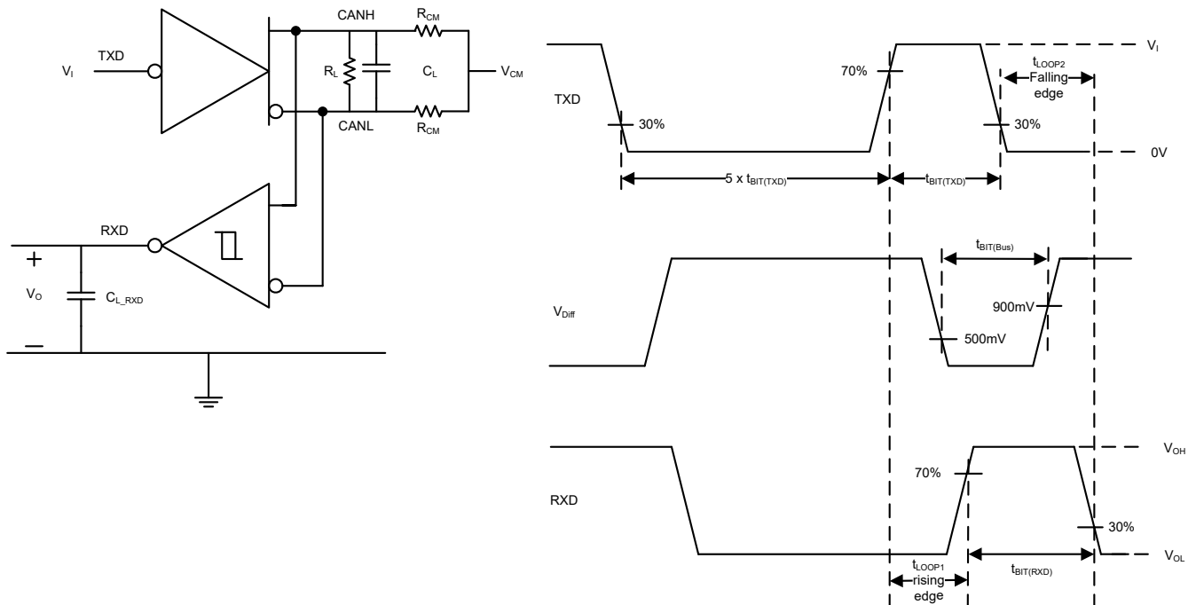
図 7-6. Transmitter and Receiver Timing Behavior Test Circuit and Measurement
