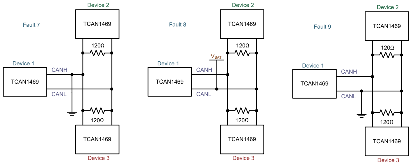
図 8-38. Fault 7, 8 and 9 Examples
