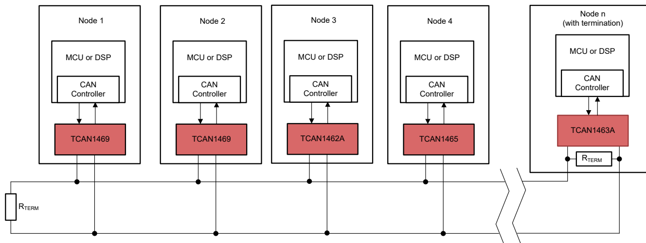
図 9-1. Typical CAN Bus
