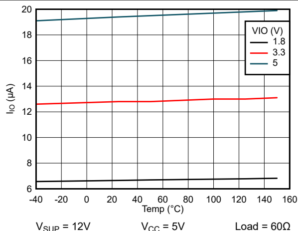
図 6-5. Normal Mode Dominant: I_{IO} vs Temperature
