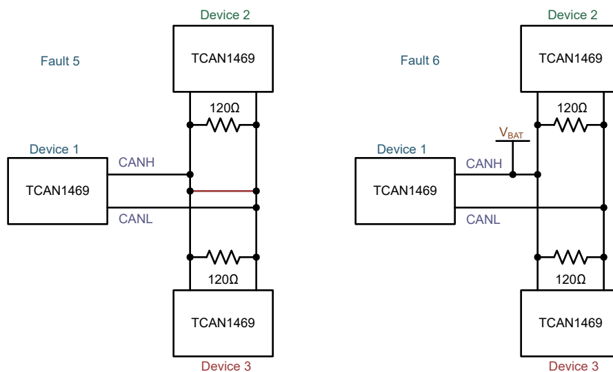
図 8-37. Fault 5 and 6 Examples
