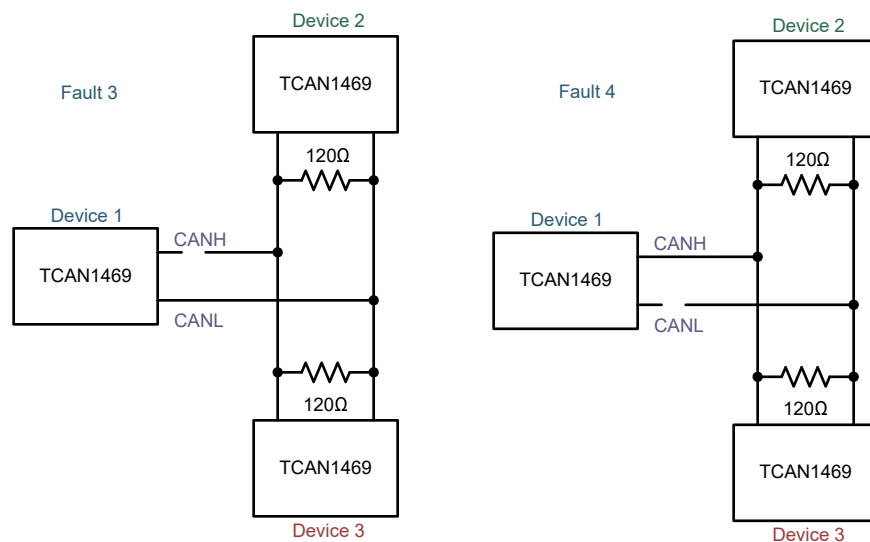
図 8-36. Open Fault 3 and 4 Examples
