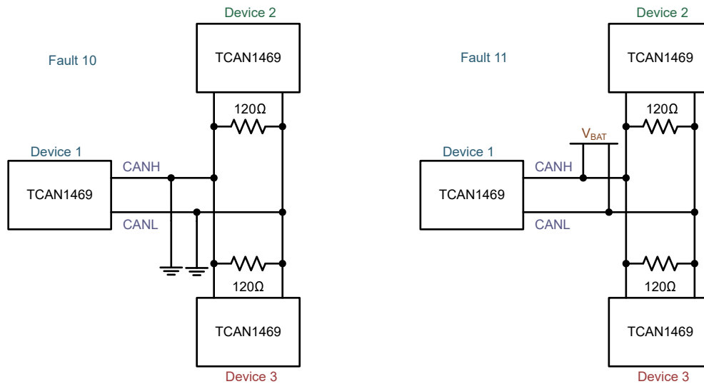
図 8-39. Fault 10 and 11 Examples
