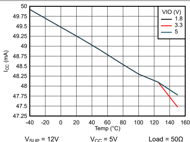
図 6-3. Normal Mode Dominant I_{CC} vs Temperature
