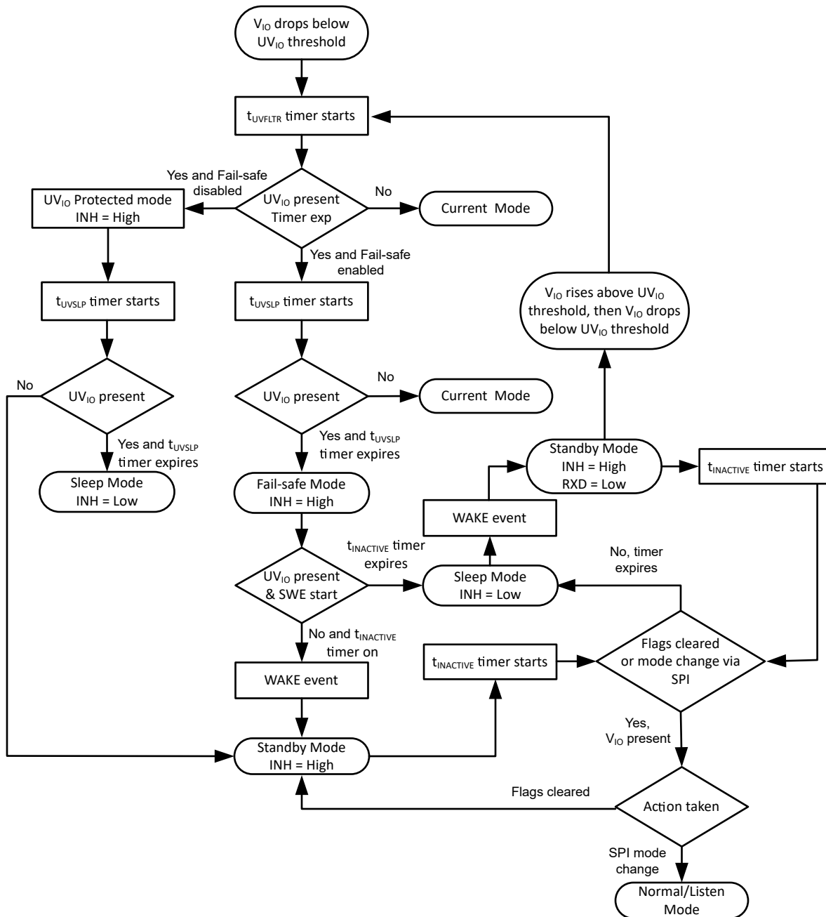
8-25. UV I0 State Diagram
