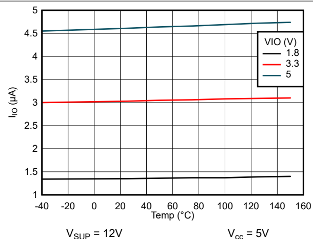
図 6-4. Normal Mode Recessive I_{IO} vs Temperature
