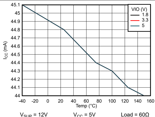
図 6-2. Normal Mode Dominant I_{CC} vs Temperature
