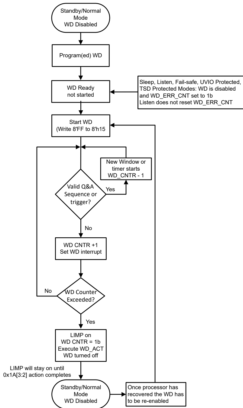
図 8-27. Watchdog Flow Chart LIMP Pin
