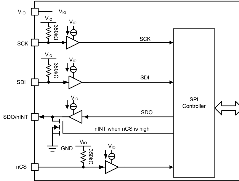
图 8-5. TCAN146x-Q1 SPI and Digital IO Block Diagram
