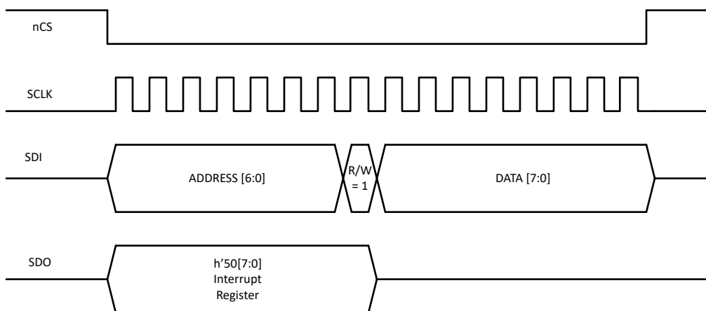
9-22. SPI Write
