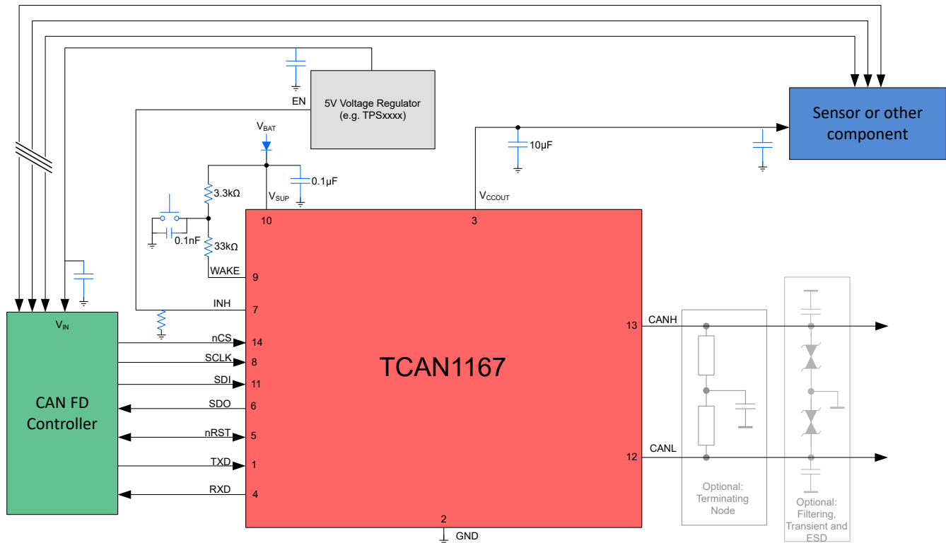
図 10-1. Typical Application
