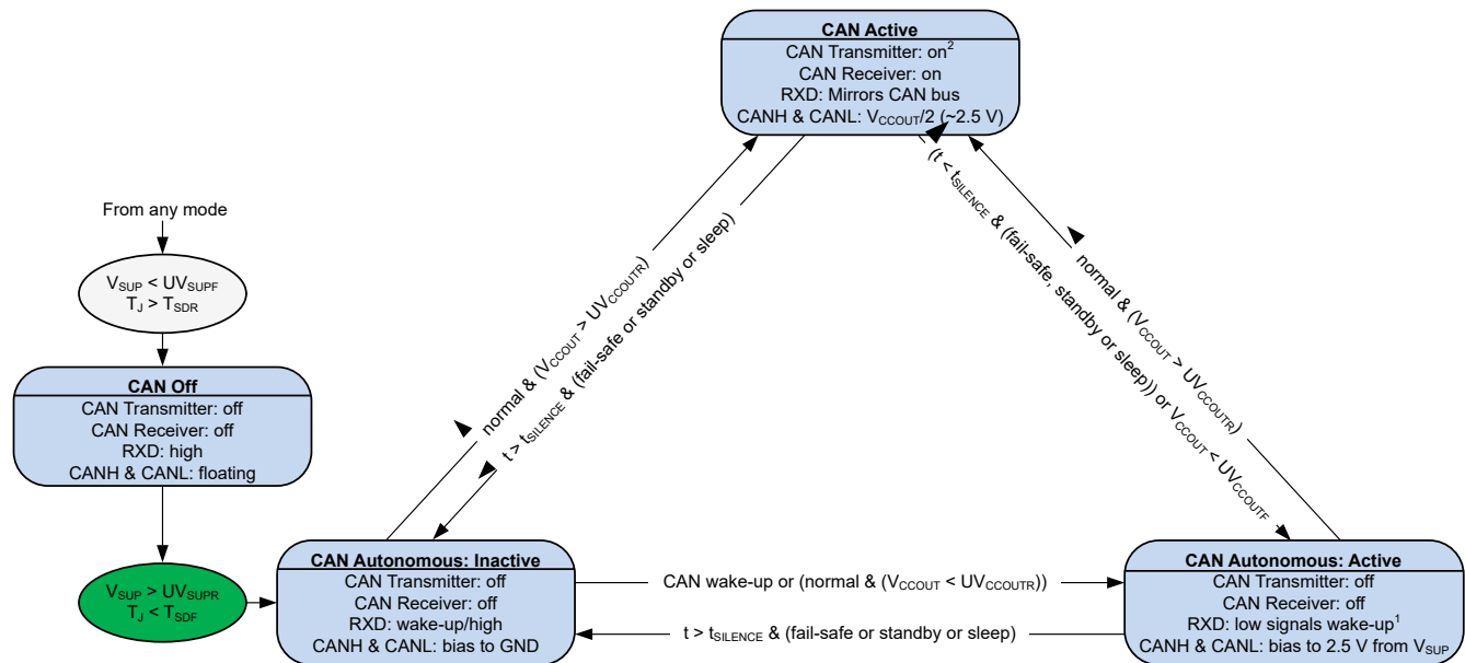
FIG 9-19. TCAN1167 CAN Transceiver State Machine
