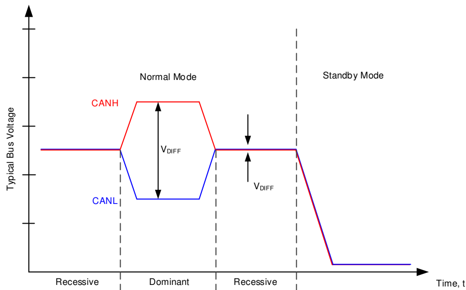
Figure 9-20. Bus States
