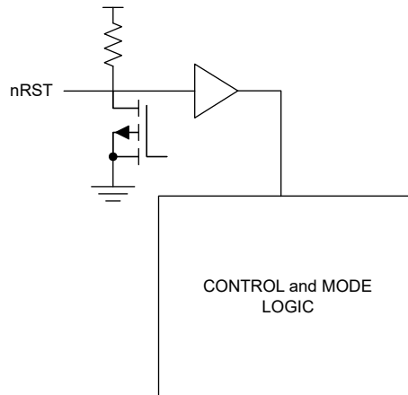
9-2. nRST Circuit
