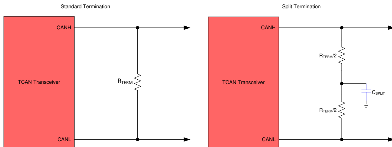
10-2. CAN Bus Termination Concepts
