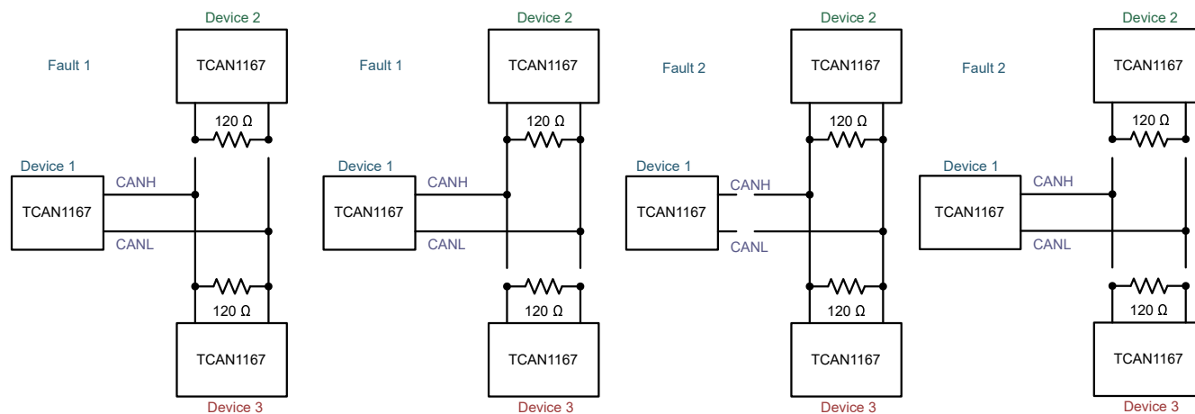
Figure 9-8. Three Node Example
