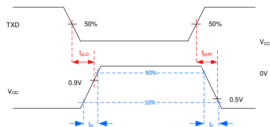
8-2. Driver Test Circuit and Measurement
