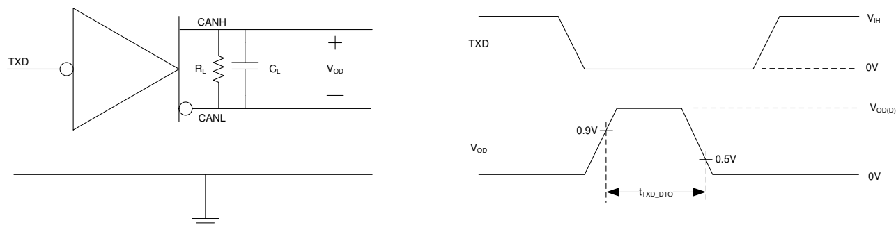
8-7. TXD Dominant Timeout Test Circuit and Measurement
