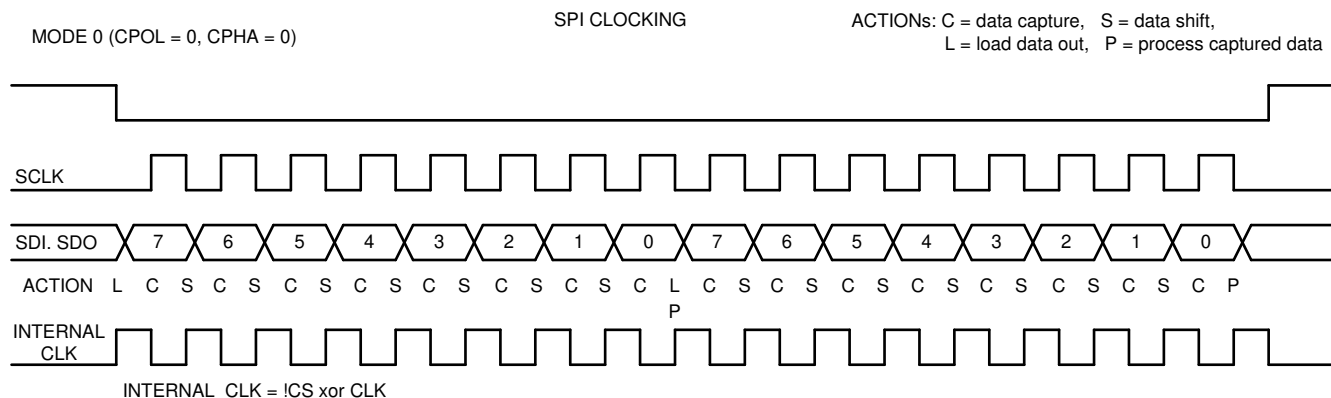
9-21. SPI Clocking
