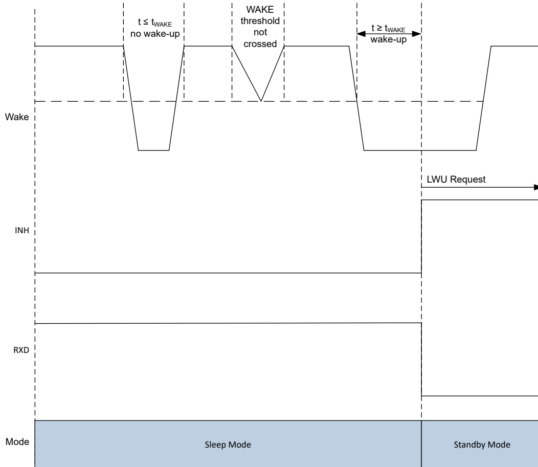
9-18. LWU Request Falling Edge
