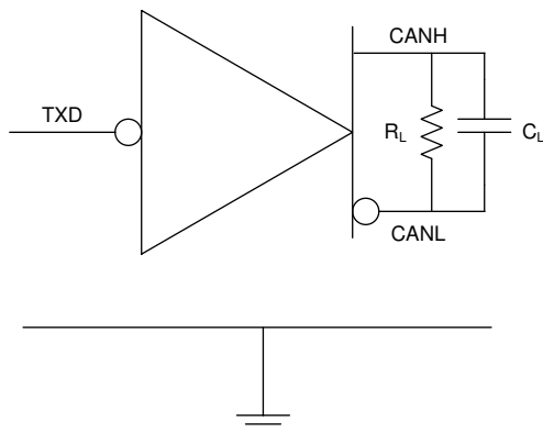
8-1. I_{SUP} Test Circuit
