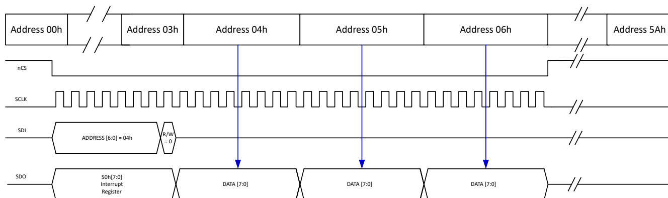
9-25. 32-bit SPI Burst Read
