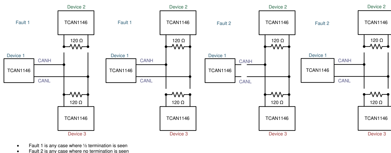
Figure 10-30. Open Fault 1 and 2 Examples
