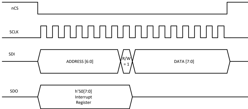
FIG 10-36. SPI Write
