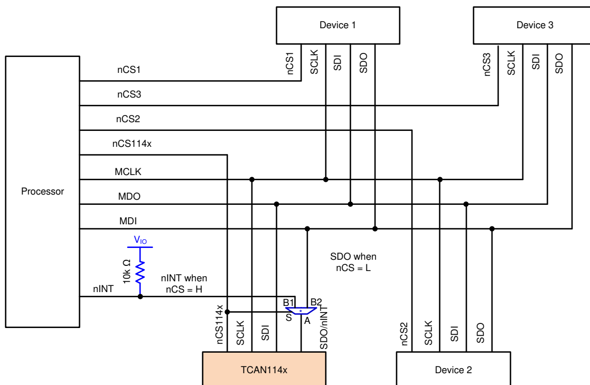
10-6. Example System Using nINT Feature
