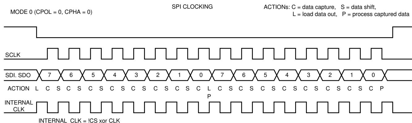
FIG 10-35. SPI Clocking
