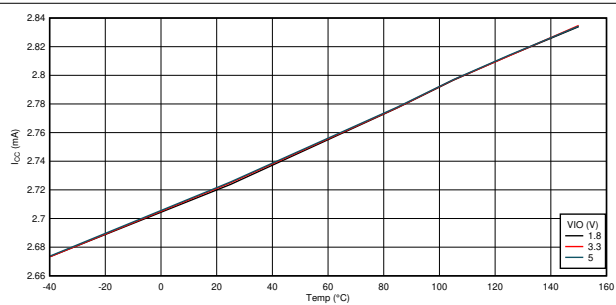
11-8. Normal Mode: I_{CC} vs Temperature Recessive
