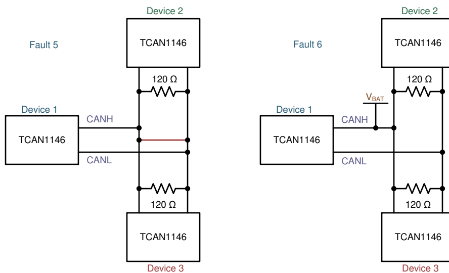
10-32. Fault 5 and 6 Examples
