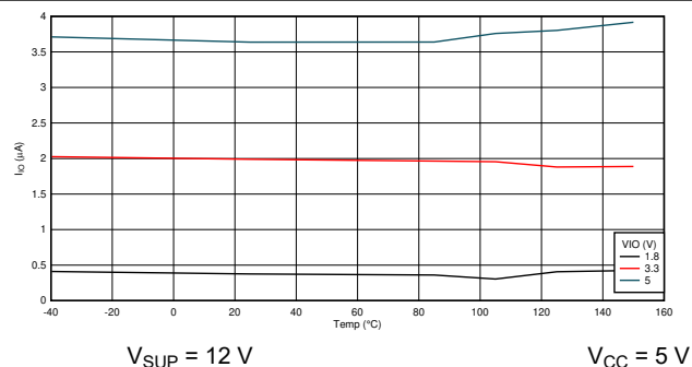
8-5. Normal Mode: I_{IO} vs Temperature Recessive
