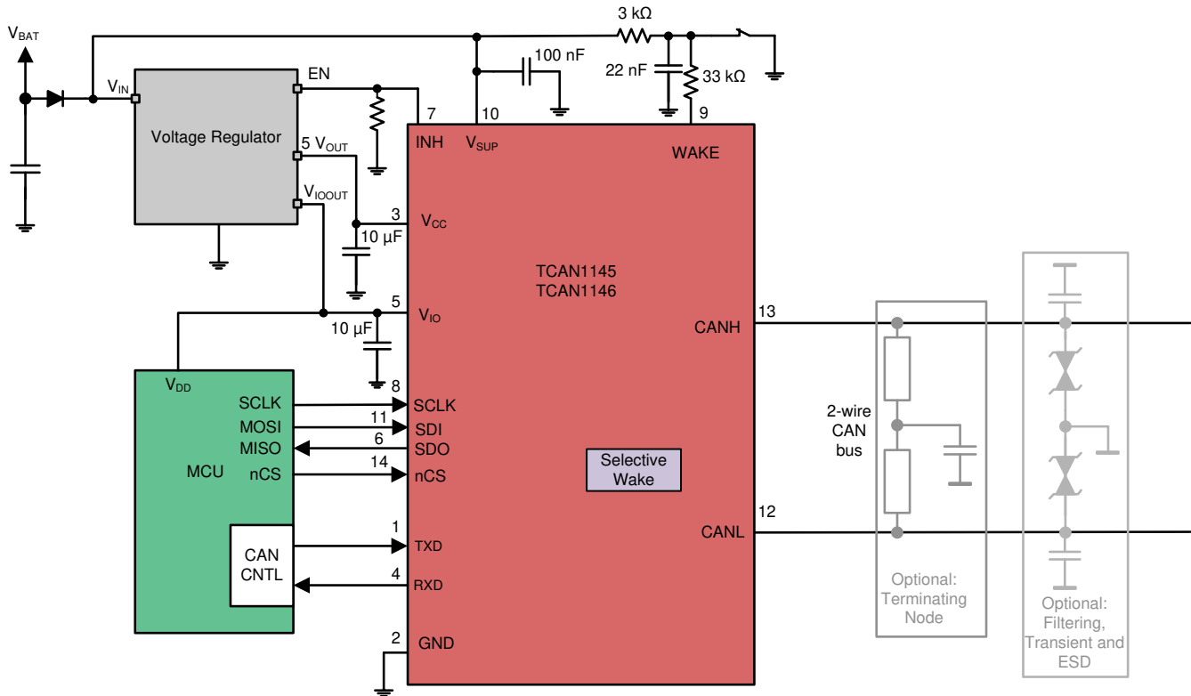
FIG 11-5. Typical CAN Applications for TCAN114x-Q1
