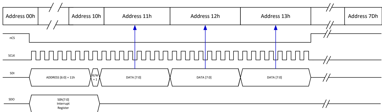
FIG 10-37. 32-bit SPI Burst Write
