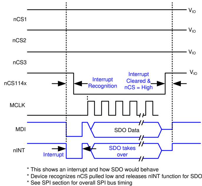
10-7. nINT Timing Diagram
