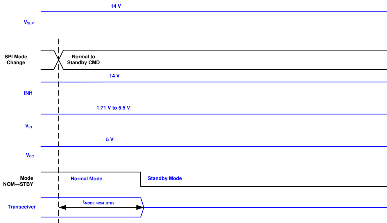
9-15. Normal to Standby Timing
