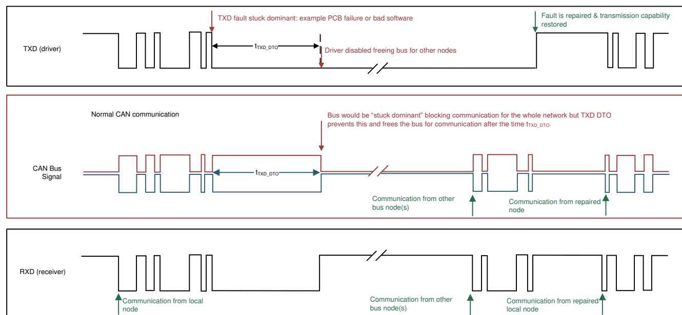
10-13. Example timing diagram with TXD DTO
