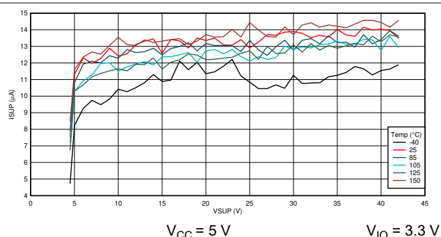
8-4. Sleep Mode: I_{SUP} vs Temperature
