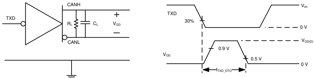
Figure 9-7. TXD Dominant Time Out Test Circuit and Measurement
