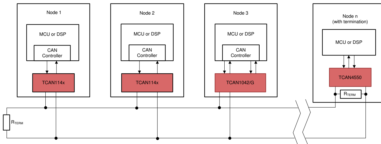
11-1. Typical CAN Bus
