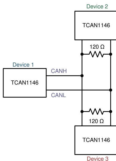
Figure 10-29. Three-Node Example
