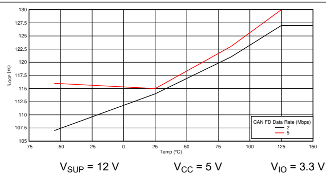
8-3. t_{LOOP} vs Temperature
