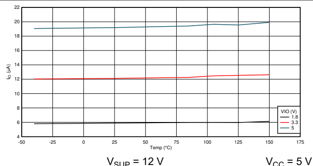
8-6. Normal Mode: I_{IO} vs Temperature Dominant
