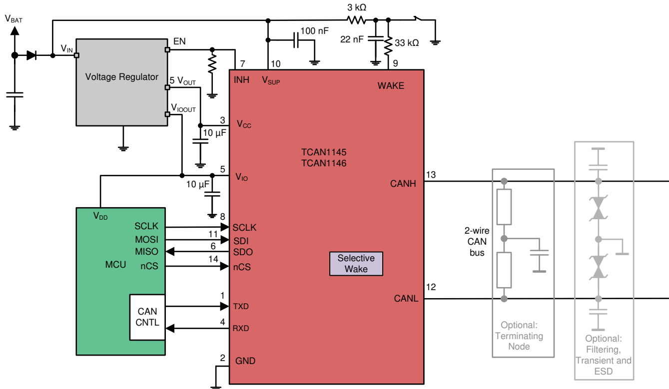
FIG 11-5. Typical CAN Applications for TCAN114x-Q1
