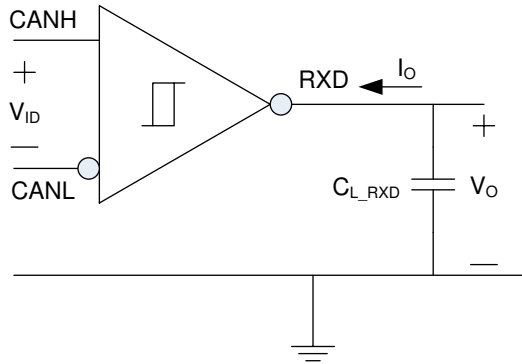
图 7-2. Receiver Test Circuit and Measurement
