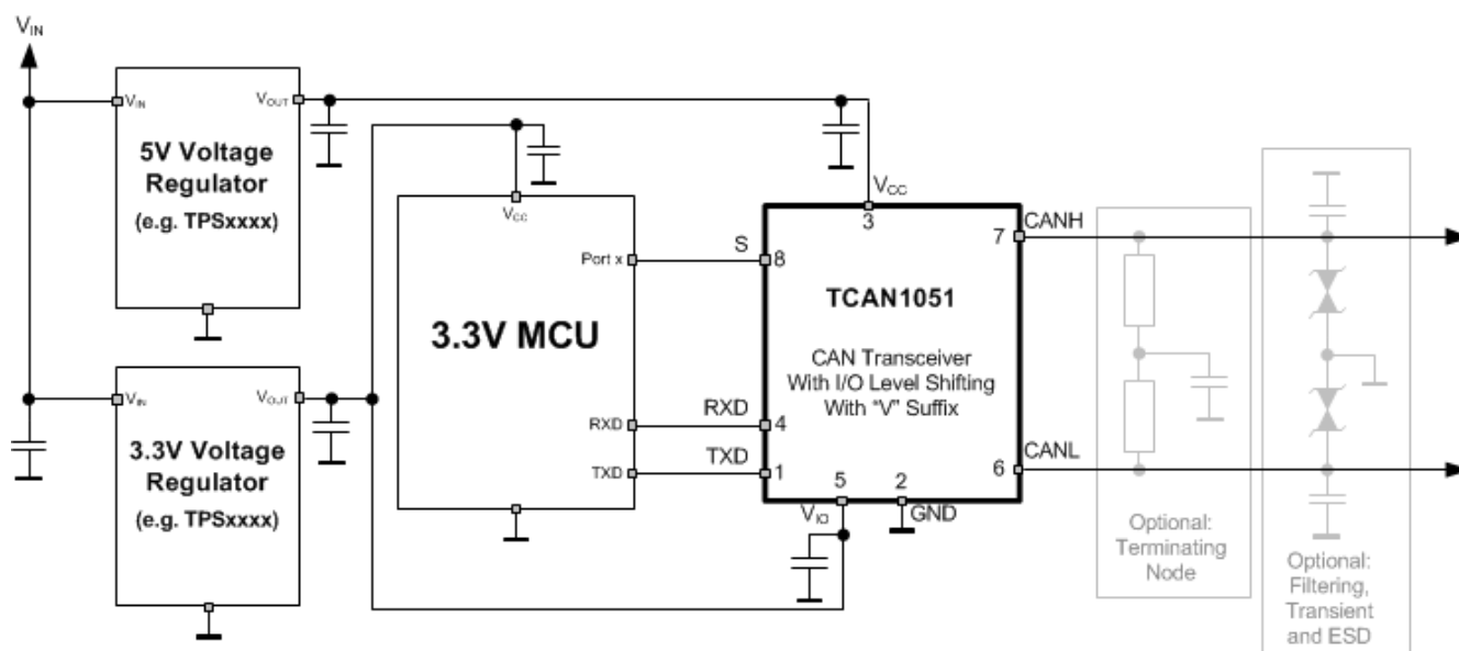
FIG 9-4. Typical CAN Bus Application Using 3.3 V CAN Controller
