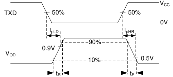
图 7-1. Driver Test Circuit and Measurement
