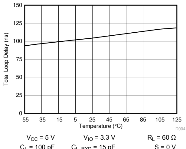
Figure 6-4. Total Loop Delay over Temperature
