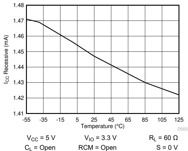
Figure 6-3. I_{CC} Recessive over Temperature
