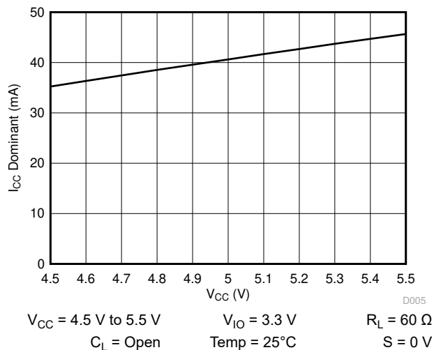
图 9-5. I_{CC} Dominant Current over V_{CC} Supply Voltage
