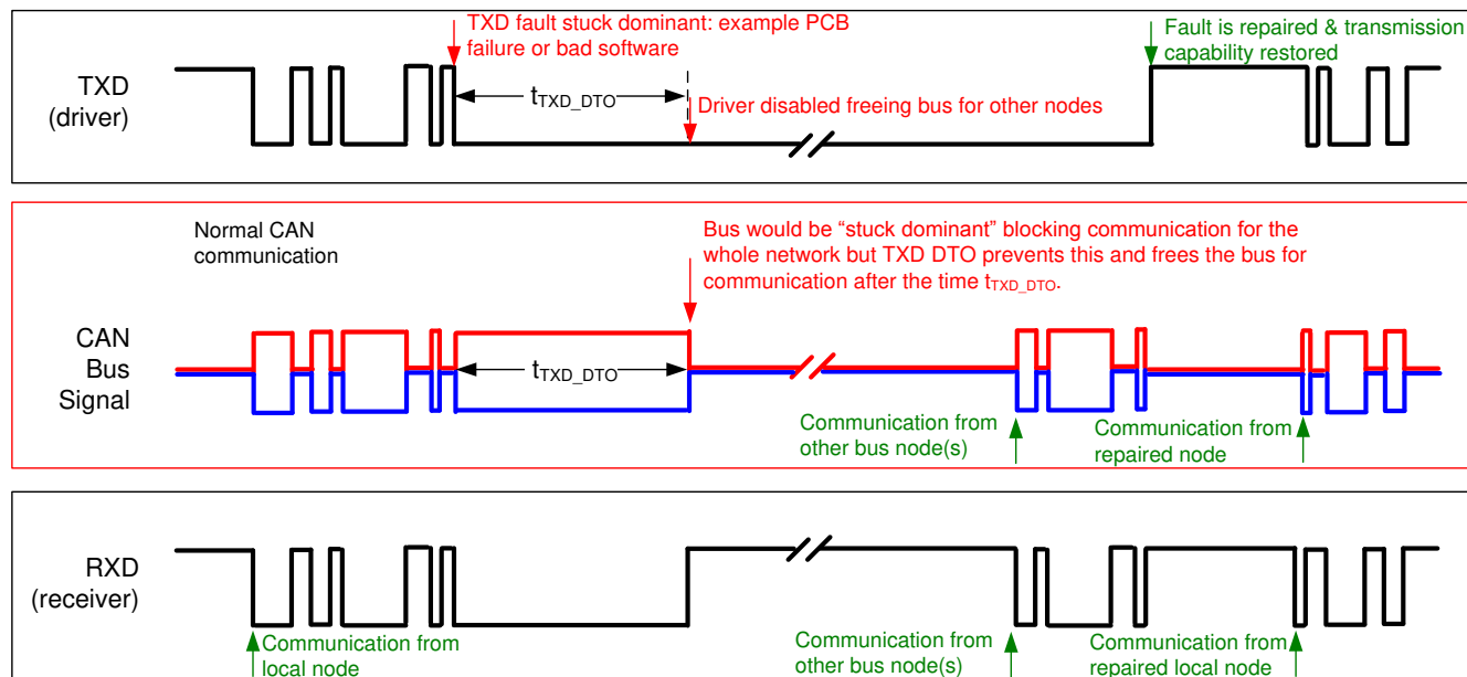
图 8-1. Example Timing Diagram for TXD DTO
