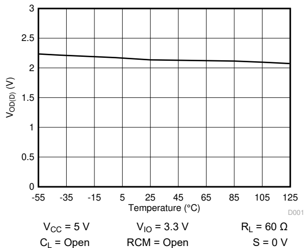
Figure 6-1. V_{OD(D)} over Temperature
