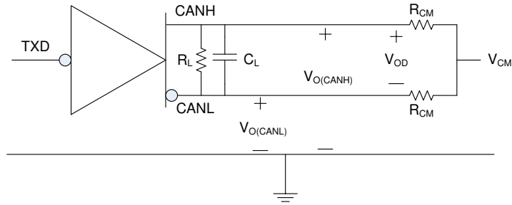
图 7-1. Driver Test Circuit and Measurement
