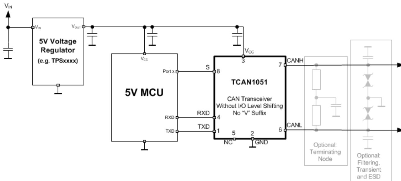
FIG 9-3. Typical CAN Bus Application Using 5 V CAN Controller
