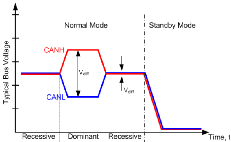
✎ 8-2. Bus States (Physical Bit Representation)
