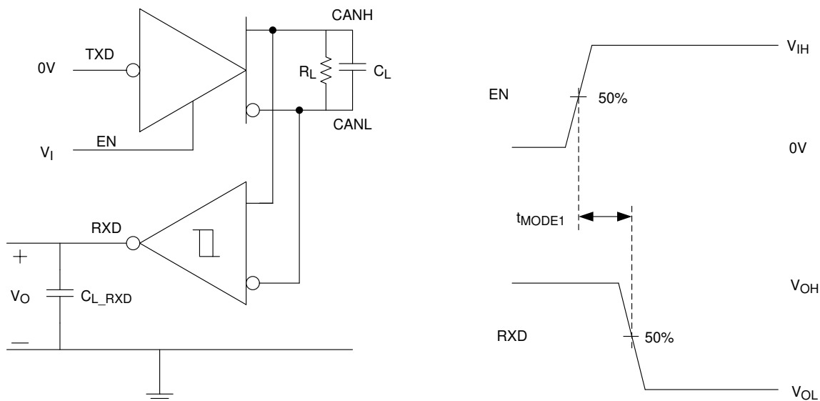
図 7-4. t_{\text{MODE1}} Test Circuit and Measurement, Silent Mode to Normal Mode
