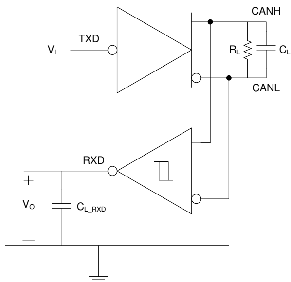
図 7-6. t_{\text{PROP(LOOP)}} Test Circuit and Measurement
