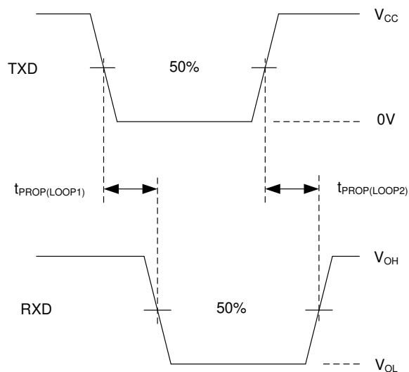
図 7-6. t_{\text{PROP(LOOP)}} Test Circuit and Measurement
