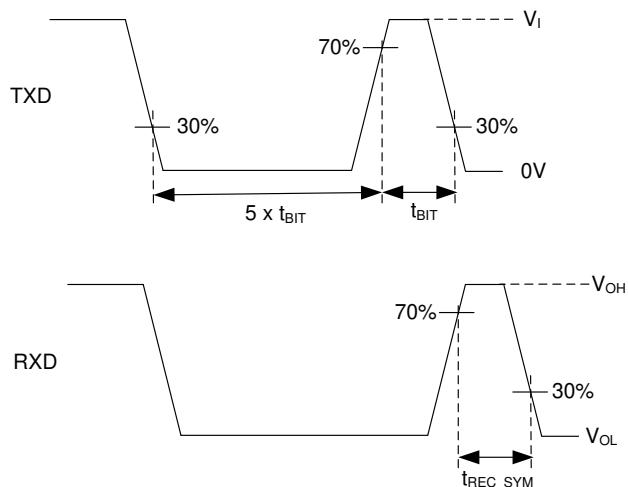
图 7-8. Loop Delay Symmetry Test Circuit and Measurement
