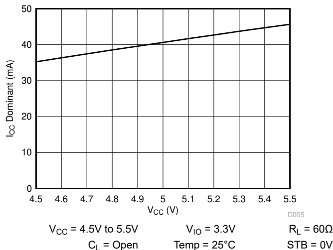
FIG 9-5. I CC Dominant Current over V CC Supply Voltage
