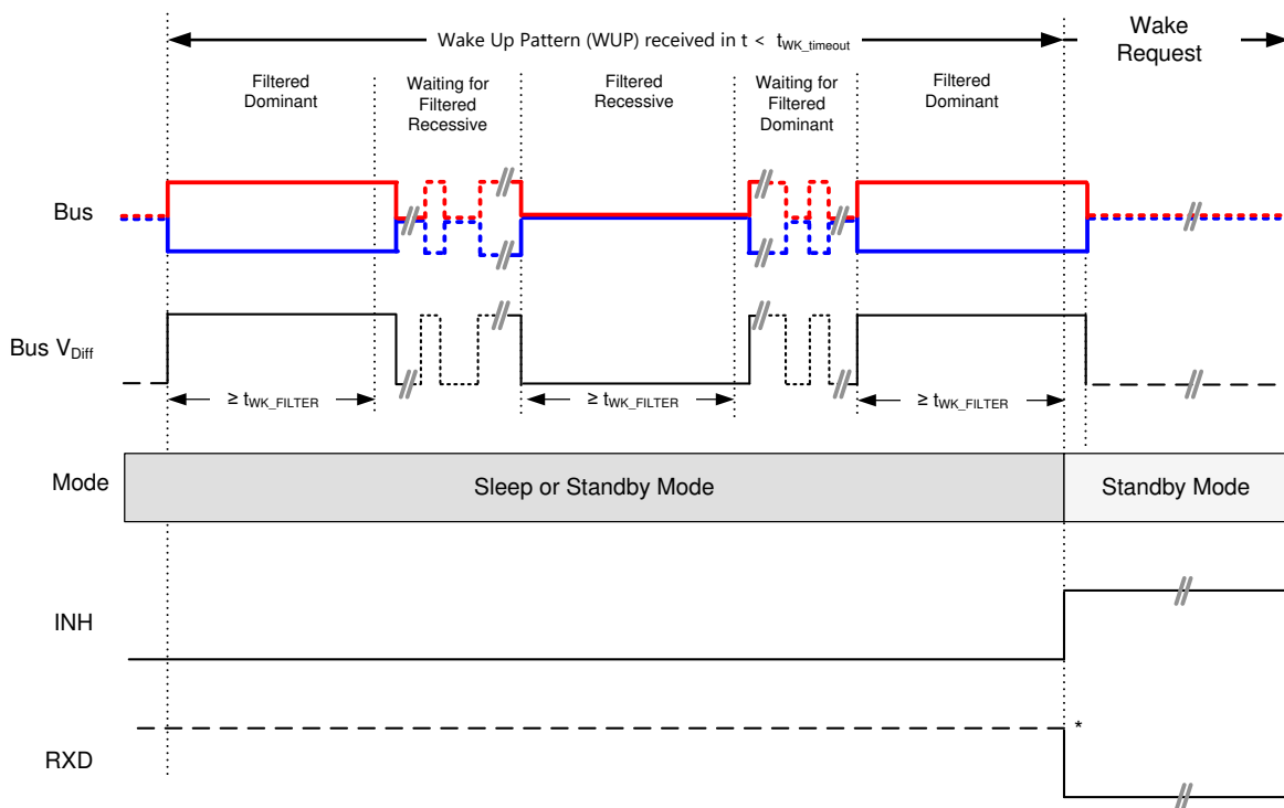
図 8-5. Wake Up Pattern (WUP)
