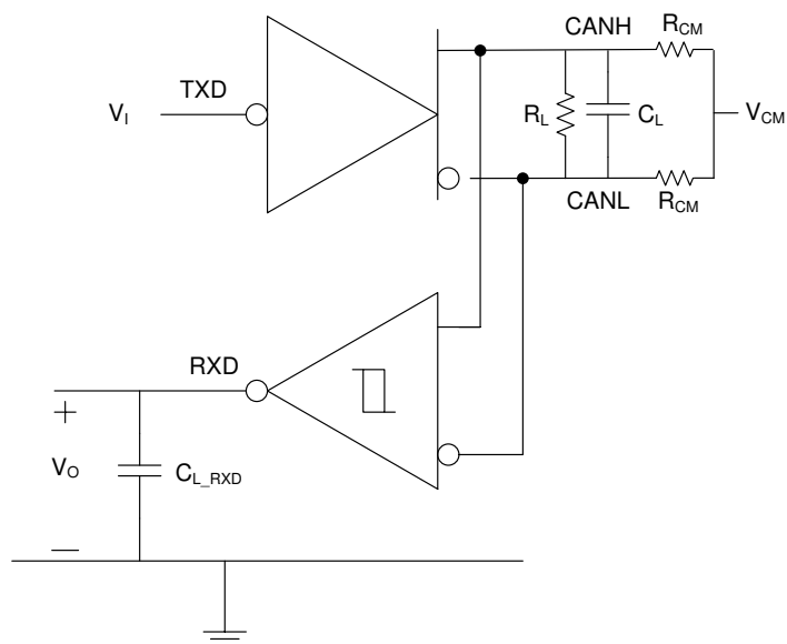
図 7-6. t_{\text{PROP(LOOP)}} Test Circuit and Measurement
