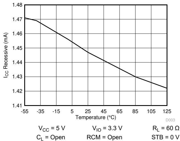
7-3. I_{CC} Recessive over Temperature
