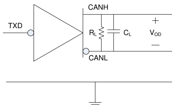
8-5. CAN FD Timing Parameter Measurement
