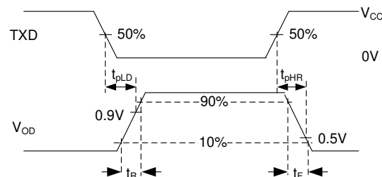
图 8-1. Driver Test Circuit and Measurement
