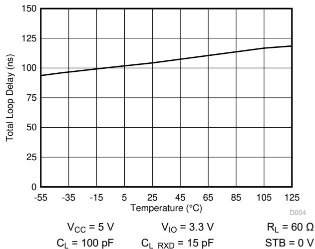
7-4. Total Loop Delay over Temperature
