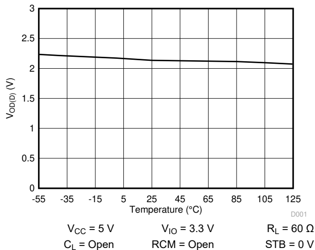
7-1. V_{OD(D)} over Temperature
