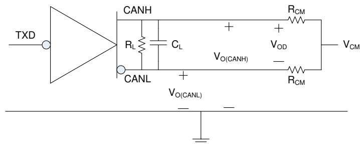
图 8-1. Driver Test Circuit and Measurement
