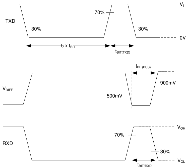
8-5. CAN FD Timing Parameter Measurement
