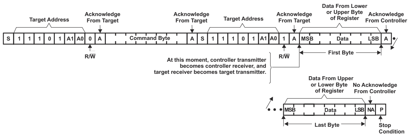
FIG 8-10. Read From Register
