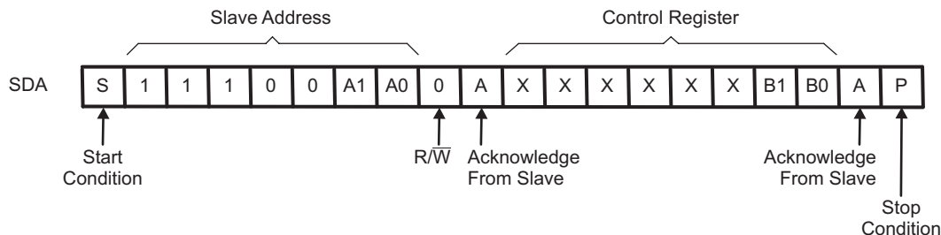
Figure 12. Write Control Register
