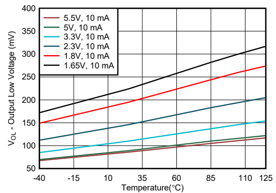
FIG 6-6. V_{OL} vs Temperature for Different V_{CC}
