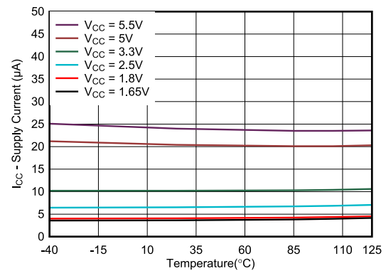
FIG 6-4. Supply Current vs Temperature for Different Supply Voltage ( V_{CC} )
