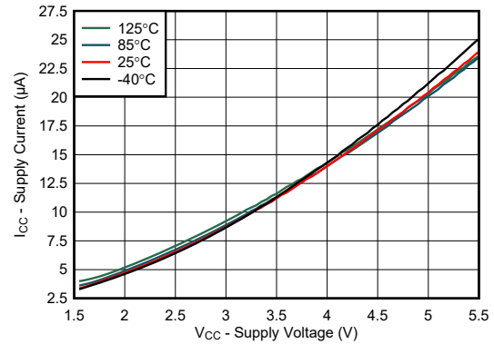
FIG 6-2. Supply Current vs Supply Voltage for Different Temperature ( T_A )
