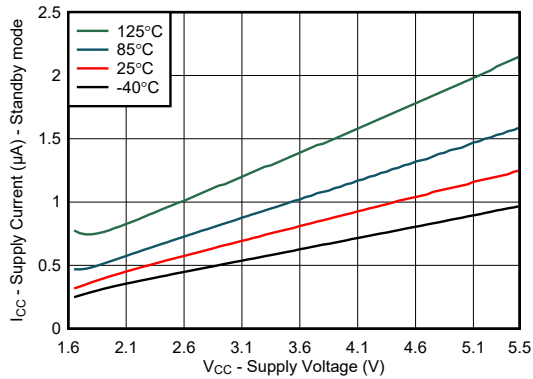
FIG 6-1. Supply Current (Standby) vs Supply Voltage for Different Temperature ( T_A )
