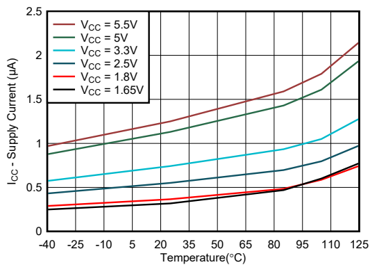
FIG 6-3. Standby Supply Current vs Temperature for Different Supply Voltage ( V_{CC} )
