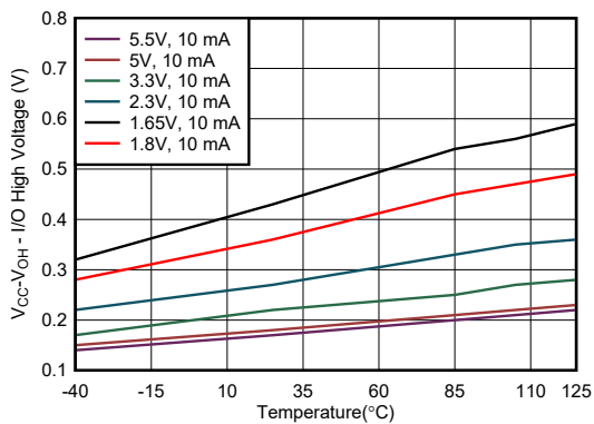
FIG 6-5. V_{CC} - V_{OH} Voltage vs Temperature for Different V_{CC}
